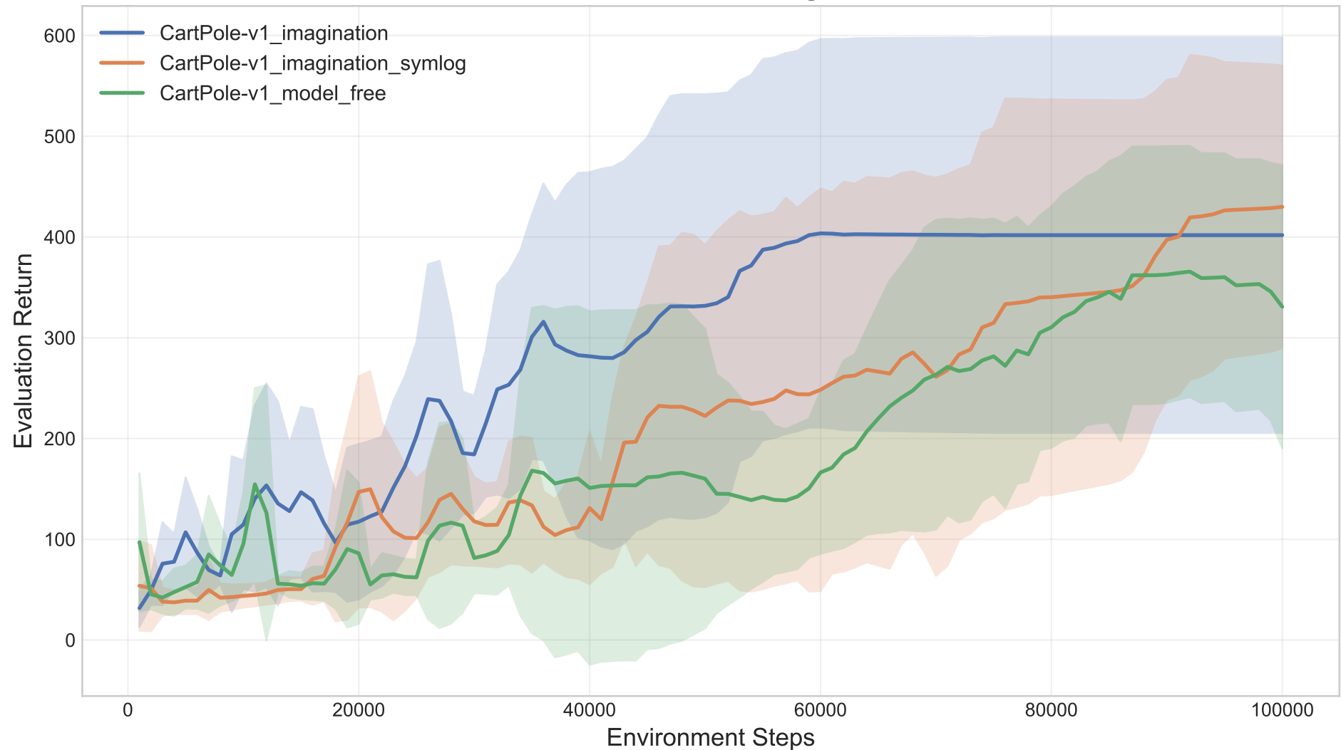
CartPole-v1 — Learning Curves
