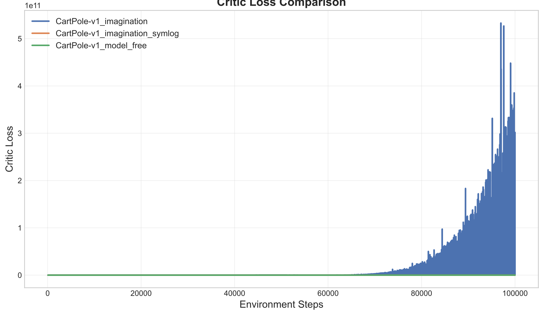
Critic Loss Comparison
