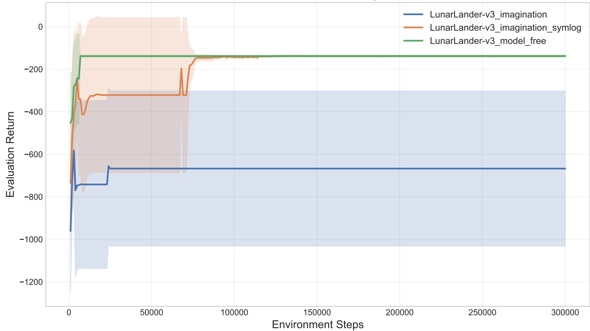
LunarLander-v3 — Learning Curves
