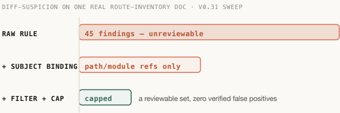
FIG. 4 — WHY A PAPER'S F1 IS THE START, NOT THE END. THE SAME RULE, THREE LEVERS LATER.
