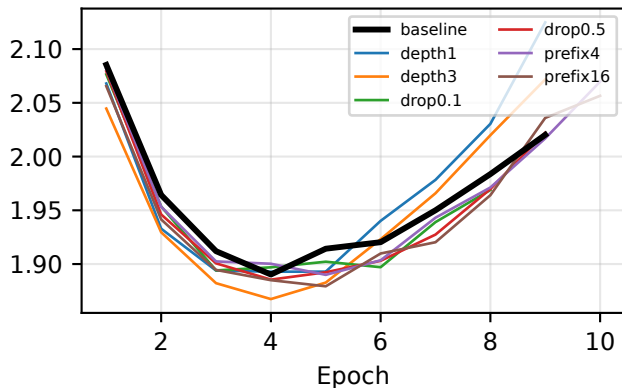
T5 -- Stage 2
