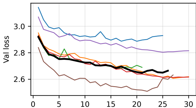
T5 -- Stage 1
