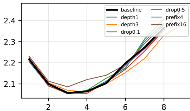
T5 -- Stage 2
