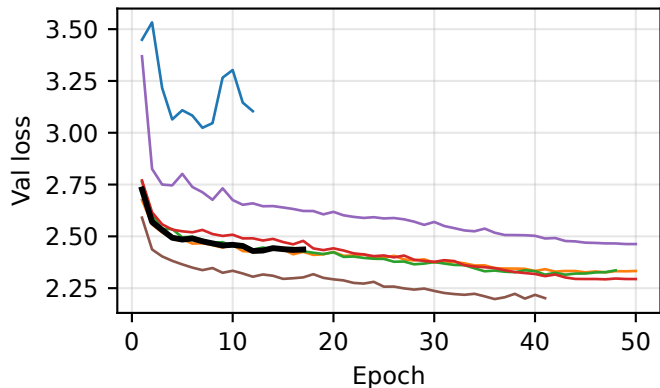
T5 -- Stage 1
