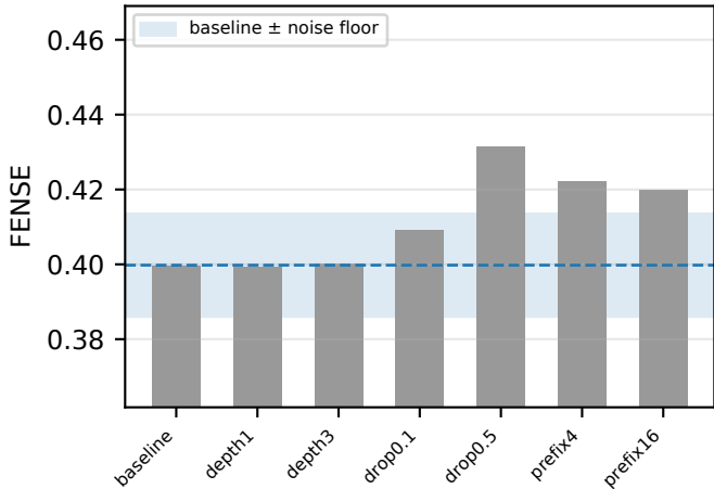
GPT-2 architecture ablations
