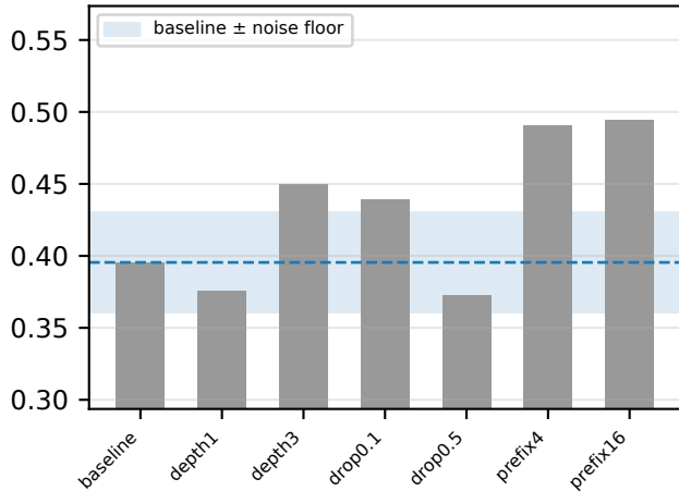
T5 architecture ablations
