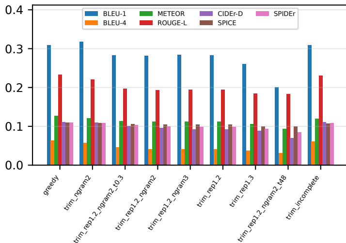
T5 -- Legacy metrics
