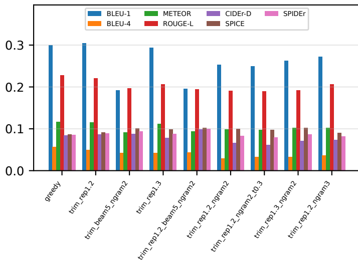
T5 -- Legacy metrics
