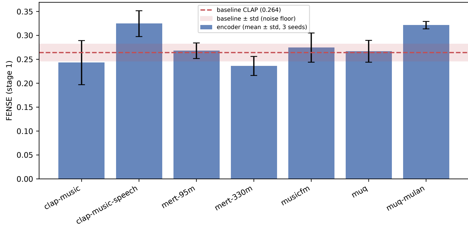
Encoder ablation vs baseline-CLAP noise floor (GPT-2 fixed)
