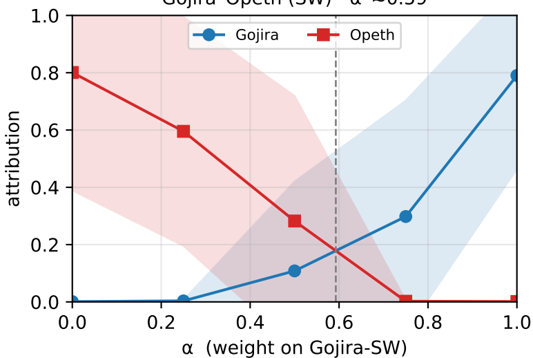
Gojira-Opeth (SW) \alpha^* \approx 0.59
