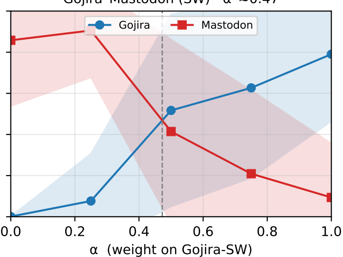
Gojira-Mastodon (SW) \alpha^* \approx 0.47
