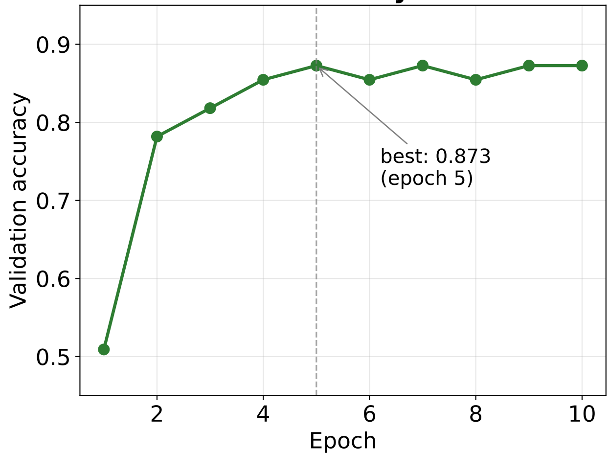
Accuracy
