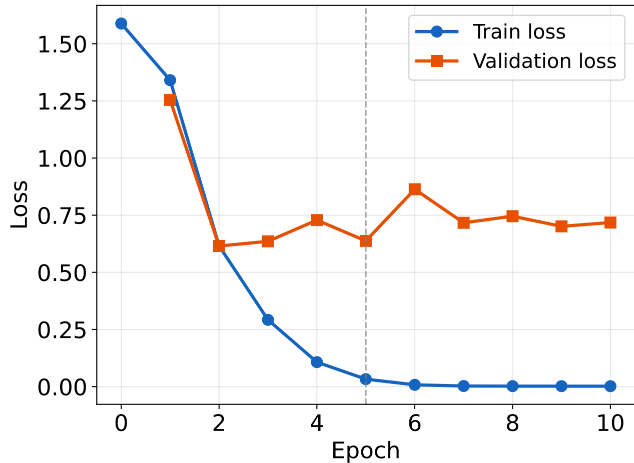
Loss
