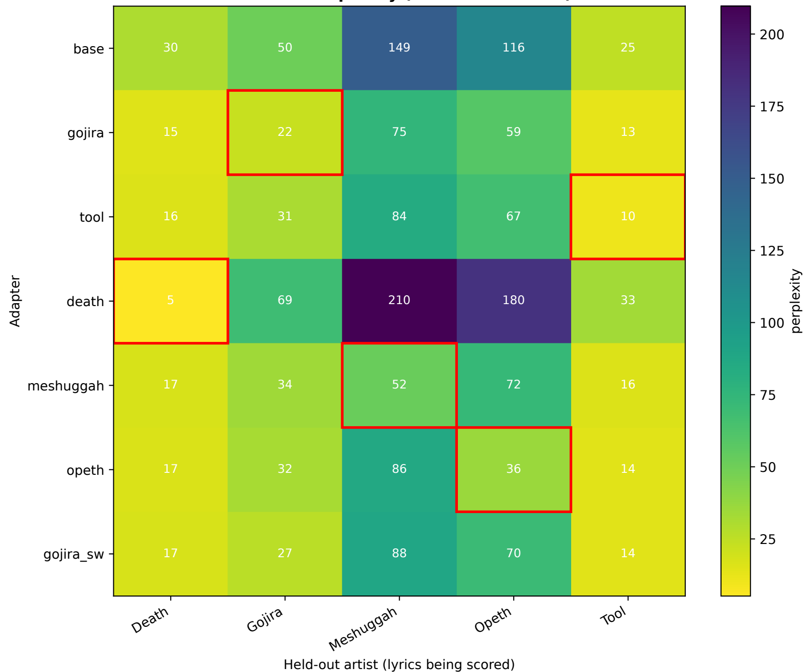
Held-out Perplexity (lower = better fit)
