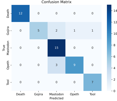
Fig. 3. Classifier confusion matrix (evaluation set, 55 songs).
