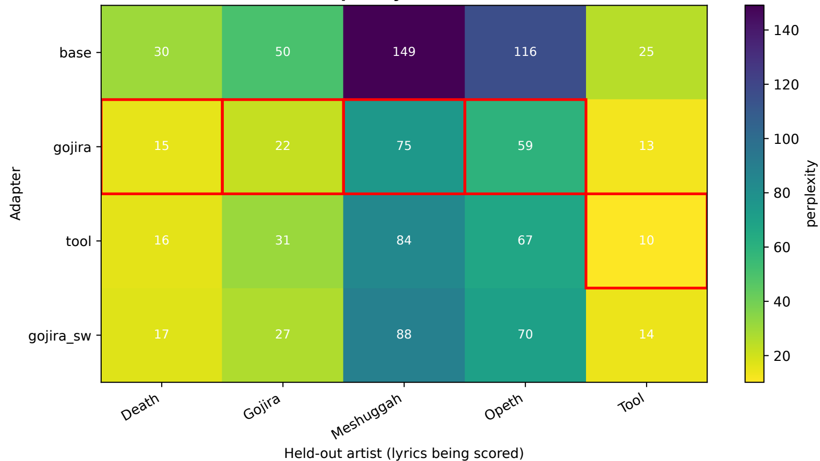
Held-out Perplexity (lower = better fit)
