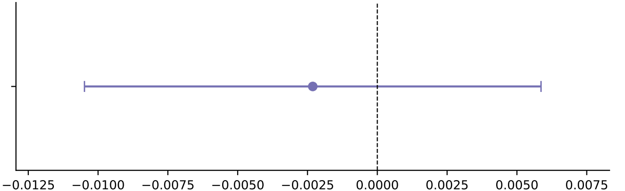
summer LST to summer NDVI adjusted built (n=89 block-years, 16 blocks)
