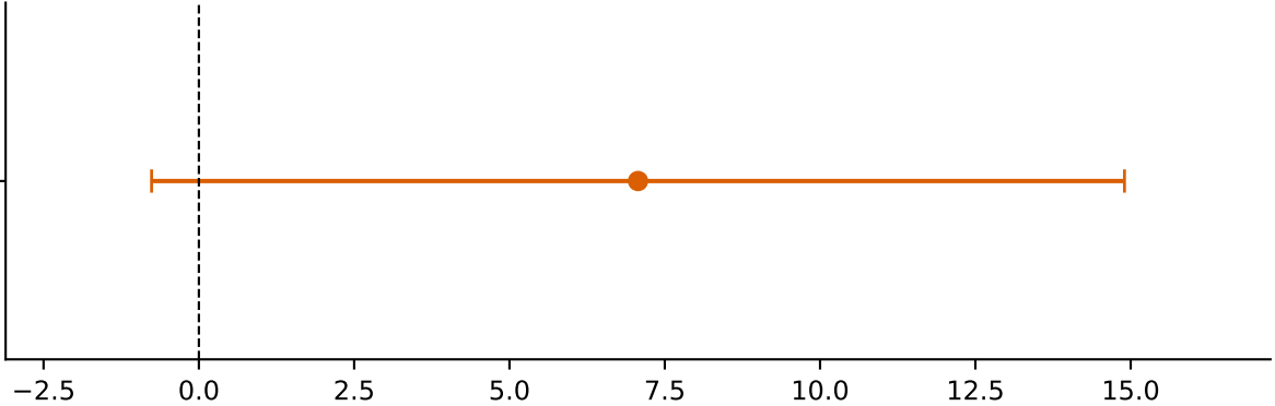
Secondary thermal consistency — built fraction → summer LST (n=89 block-years, 16 blocks)
