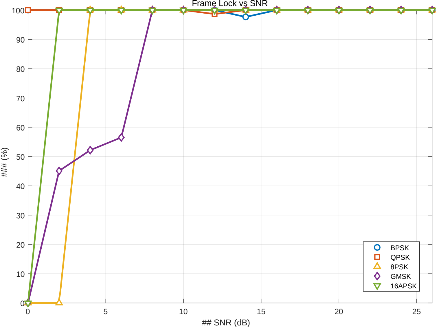
Frame Lock vs SNR
