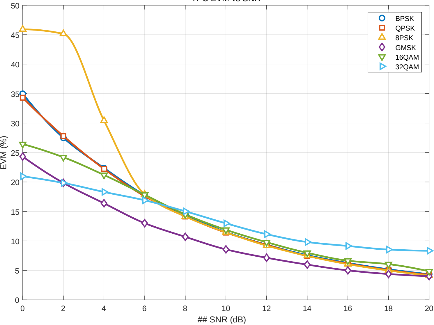
TPC EVM vs SNR
