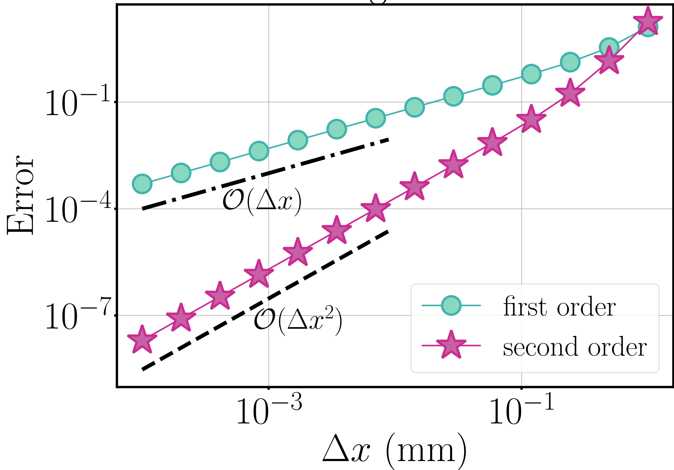
Convergence Plot
