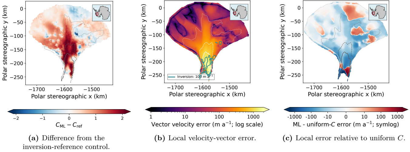
Fig. 7. Spatial evaluation of CFG02 with all of PIG withheld. Panel (a) shows the median predicted control relative to the inversion-reference control. Panel (b) shows \|\mathbf{u}_{\text{ML}} - \mathbf{u}_{\text{obs}}\| . Panel (c) shows the difference between the local CFG02 and uniform- C velocity errors; negative values indicate lower error for CFG02 and positive values indicate lower error for uniform C . Contours mark observed speeds of 100 (dotted), 500 (dashed), and 1000 \text{m a}^{-1} (solid). The cyan contour in panel (b) marks an inversion-reference velocity error of 100 \text{m a}^{-1} . Velocity fields are rendered from the original 450 m grid using display interpolation; all reported statistics use the original grid values. Both CFG02 and uniform C replace the inversion reference only inside the PIG holdout.
