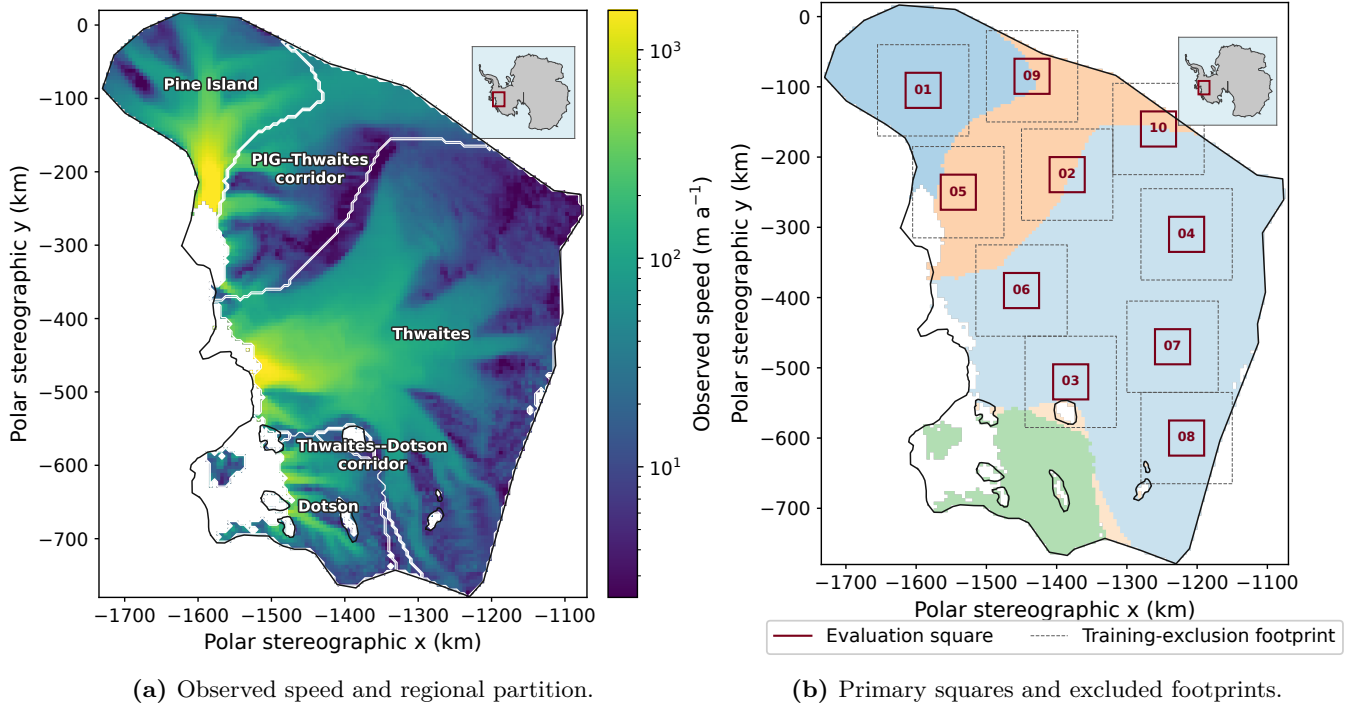
Fig. 2. Study region and holdout design. Panel (a) shows observed MEaSUREs speed over the eligible part of the Amundsen Sea sector, with the PIG, Thwaites, and Dotson regions and the two inter-catchment corridors. Panel (b) shows the ten 50 km primary evaluation squares (solid) and their 130 km excluded footprints (dashed). Each footprint includes a 40 km buffer on every side of the central square and is excluded from training and validation datasets.
