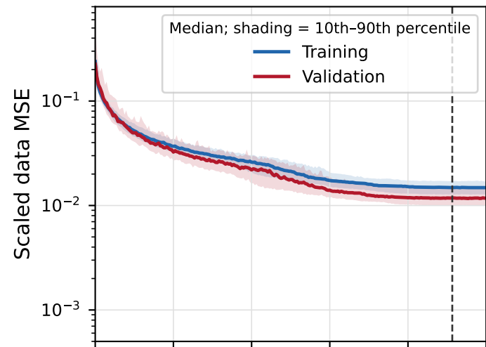
CFG04: best epoch 281 [242-321]
