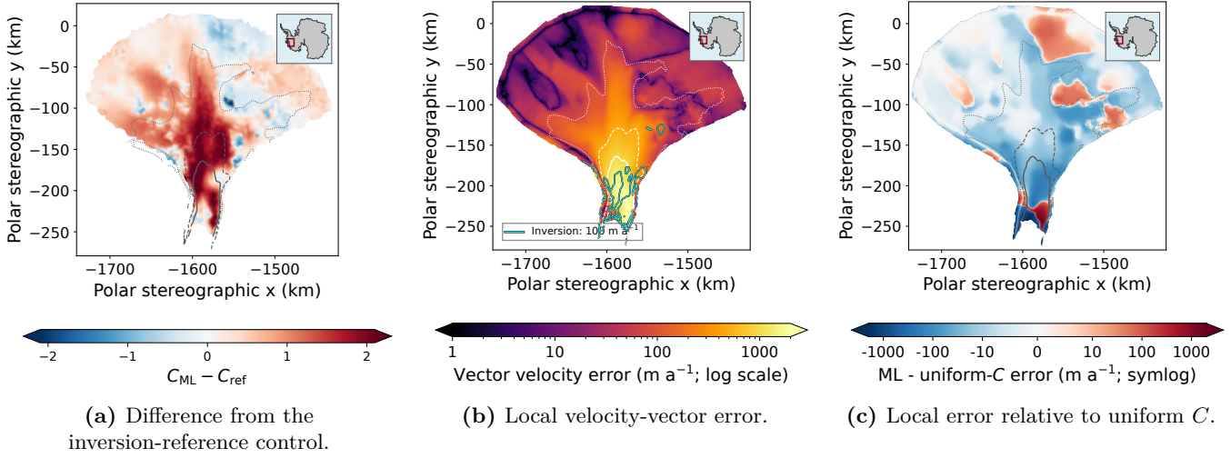
Fig. 7. Spatial evaluation of CFG02 with all of PIG withheld. Panel (a) shows the median predicted control relative to the inversion-reference control. Panel (b) shows \|\mathbf{u}_{ML} - \mathbf{u}_{obs}\| . Panel (c) shows the difference between the local CFG02 and uniform- C velocity errors; negative values indicate lower error for CFG02 and positive values indicate lower error for uniform C . Contours mark observed speeds of 100 (dotted), 500 (dashed), and 1000 \text{m a}^{-1} (solid). The cyan contour in panel (b) marks an inversion-reference velocity error of 100 \text{m a}^{-1} . Velocity fields are rendered from the original 450 m grid using display interpolation; all reported statistics use the original grid values. Both CFG02 and uniform C replace the inversion reference only inside the PIG holdout.
