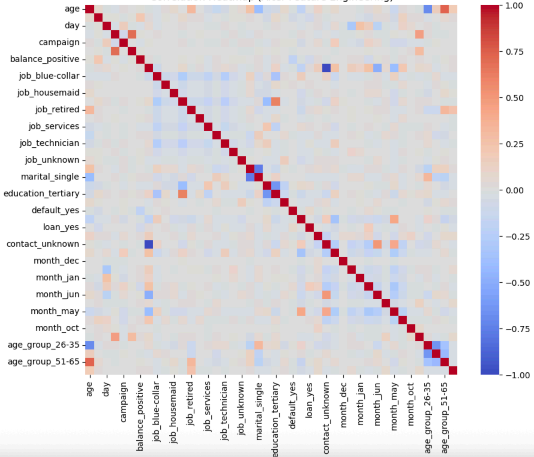
Correlation Heatmap (After Feature Engineering)
