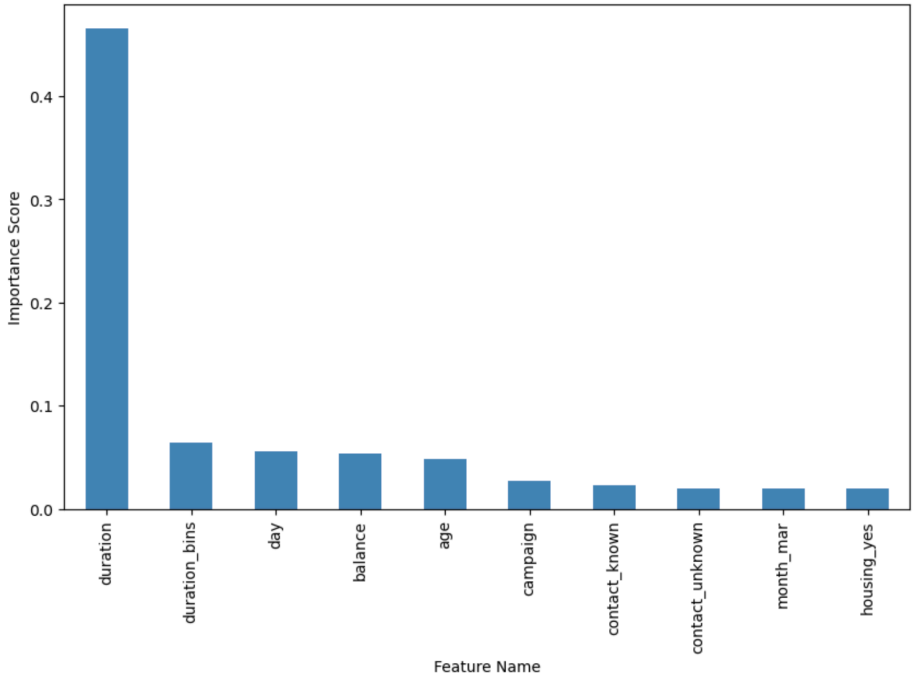
Top 10 Important Features (Random Forest)
