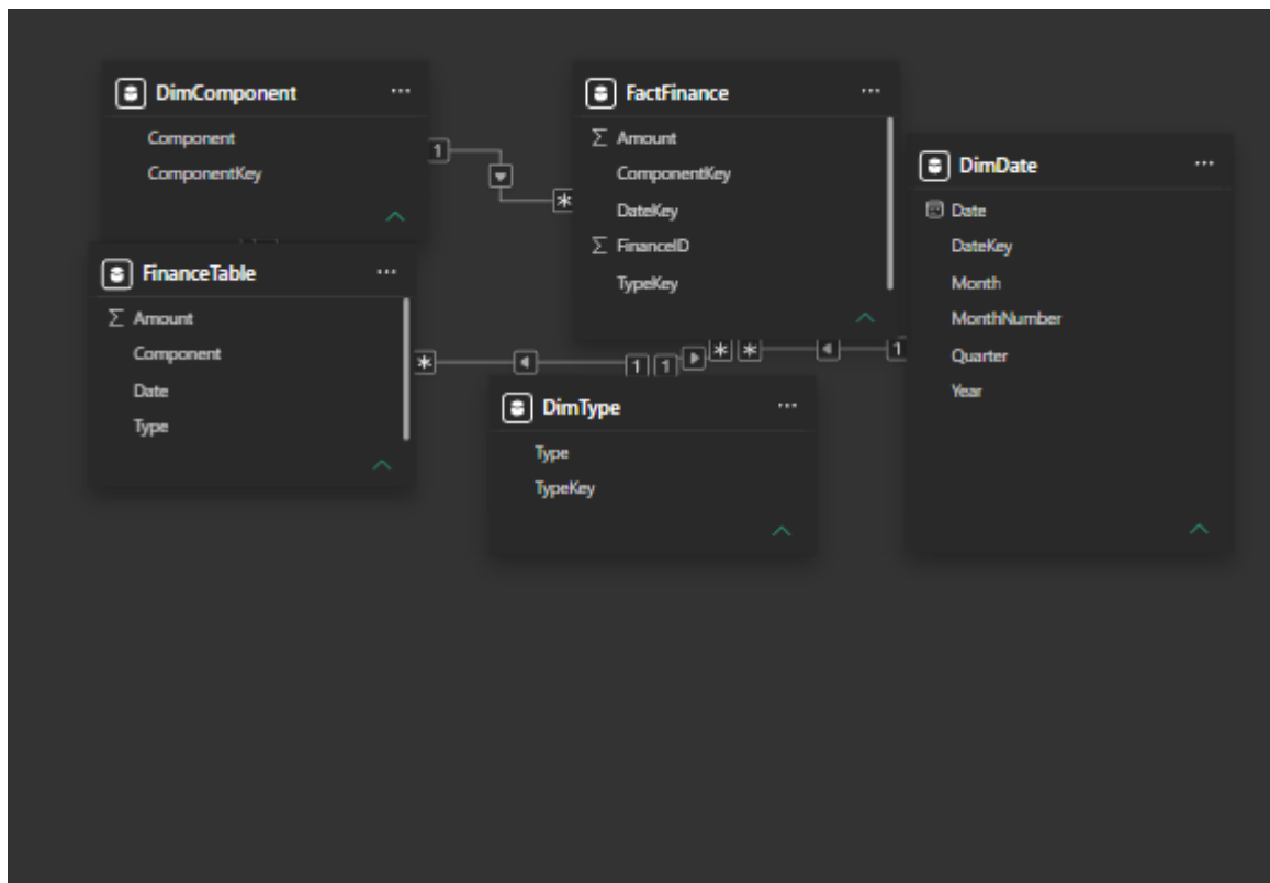
Merged FactFinance and DimComponent
