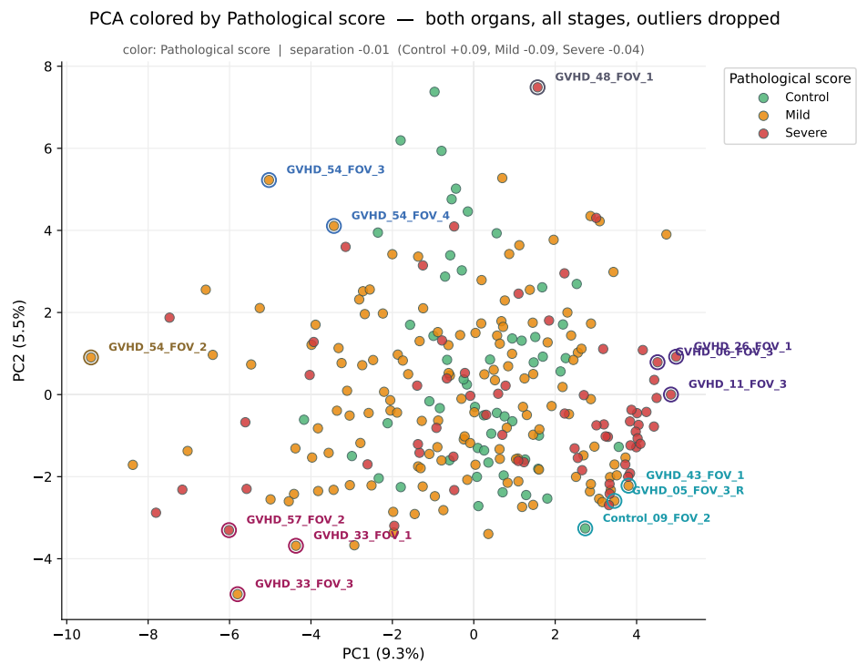
Figure 66: Values follow Figure 1.12, after the five far-out FOVs are dropped and the PCA refitted — the edges of the crowd itself.
