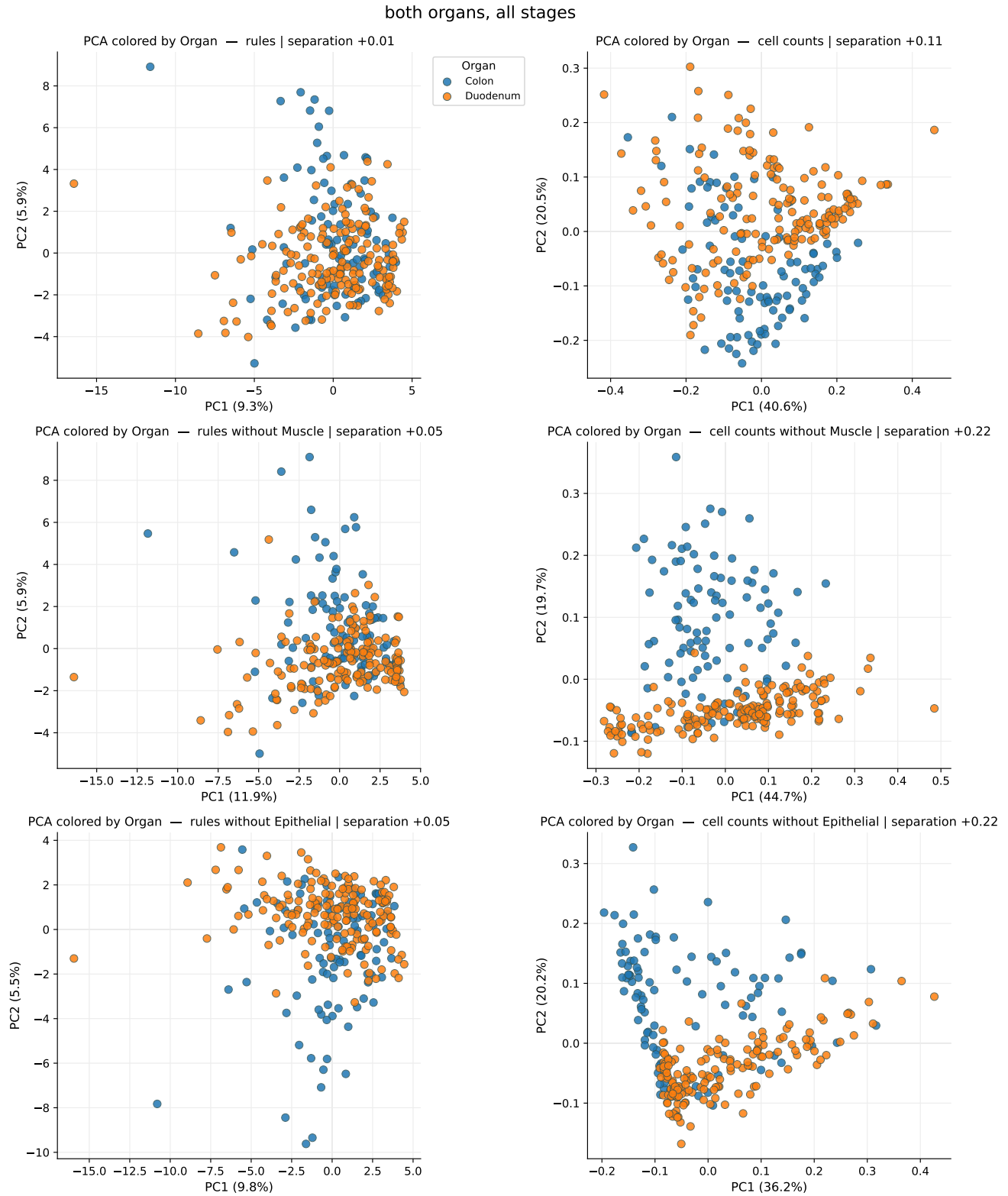
Figure 32: Top row: the FOVs placed by their rules (left) and by their cell composition alone (right), no rules involved. Each row below repeats the pair with one composition-linked cell type removed — its rules dropped on the left, its column dropped on the right. Removing them one at a time, rather than together, shows whether a single cell type carries the separation. Each panel title gives what it was built from and its own separation number.
