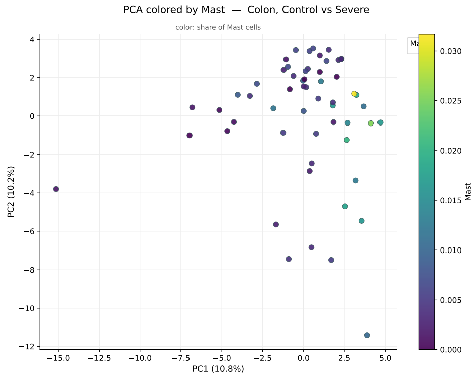
Figure 42: Values follow Figure 1.9, for this scope.
