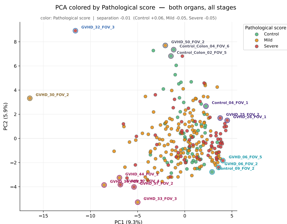
Figure 64: The PCA with the corner FOVs named and circled. A corner is found by standing at the median, looking in one of eight directions, and taking the FOV furthest ahead. Both axes are first divided by their own spread, so the wider component does not decide every direction. Two corners closer together than 15% of the cloud's width count as one. Label and ring colours mark which corner a FOV belongs to, and the maps below use the same colours.
