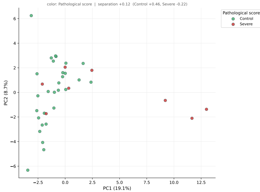
Figure 58: A fresh PCA on group A alone: 37 duodenal FOVs alike in composition, 29 Control and 8 Severe. Separation +0.124, and lopsided — Control +0.46, Severe -0.22. Eight FOVs are too few to form a group, so this figure shows a recognisable healthy state rather than two stages coming apart.
