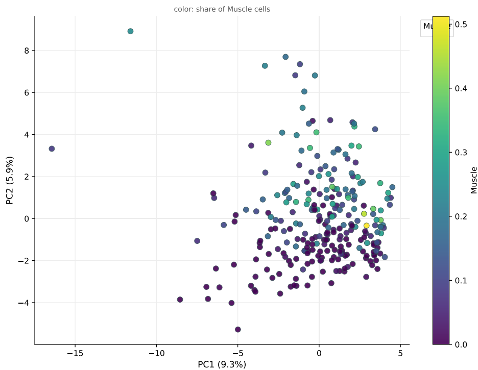
Figure 39: The same PCA coloured by the share of the two cell types whose correlation with the components was strongest. A smooth colour gradient across the plot means the component is largely tracking how common that cell type is.
