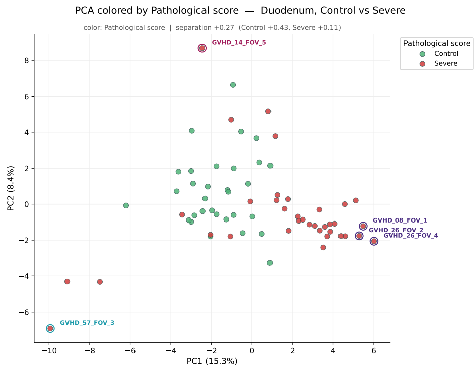
Figure 70: Values follow Figure 1.12; duodenum, Control against Severe. Five corners.
