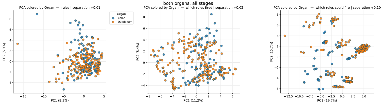
Figure 35: Three matrices over the same FOVs and the same rules. Left: the lift values. Middle: the same rules reduced to found or not found, values thrown away. Right: whether the FOV held enough of both of a rule's cell types for that rule to be findable at all — at least 15 cells of a type and at least 1% of the FOV, the floor the mining itself used. The right panel carries no information about position.
