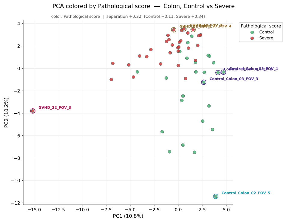
Figure 68: Values follow Figure 1.12; colon, Control against Severe. Eight corners, half of them control FOVs.
