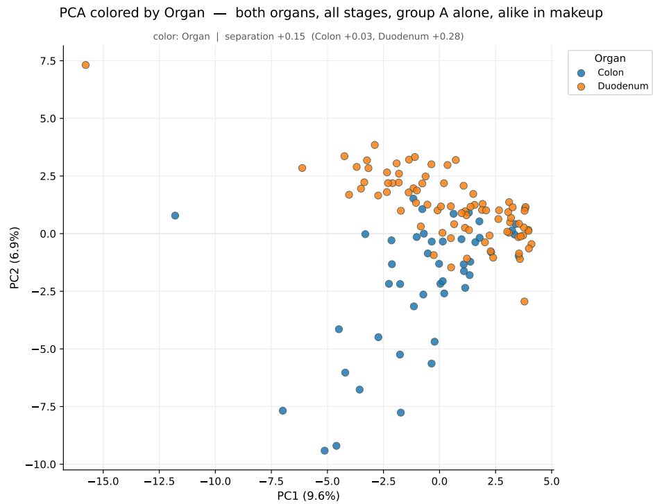
Figure 50: A fresh PCA on group A alone — 128 FOVs alike in composition, 47 colon and 81 duodenum. This is a new PCA, not the earlier one redrawn, so its axes are its own. Separation +0.154 (Colon +0.03, Duodenum +0.28), against +0.009 for all FOVs together.
