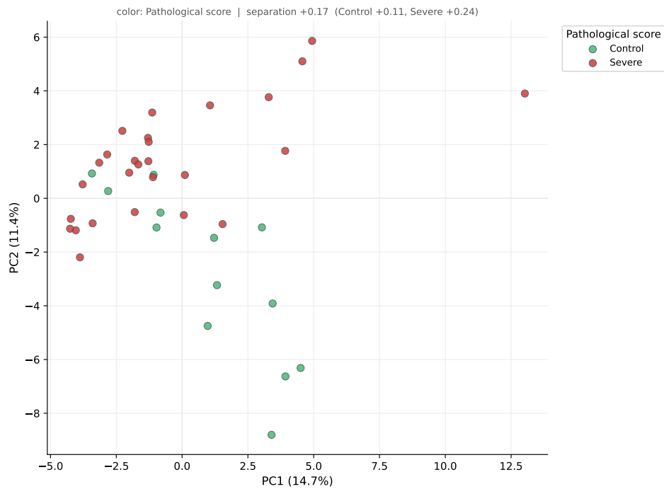
Figure 54: A fresh PCA on group B alone: 40 colonic FOVs alike in composition, 13 Control and 27 Severe. Separation +0.173 (Control +0.11, Severe +0.24) — below the +0.223 the same scope reaches on all its FOVs, but with both groups still scoring.
