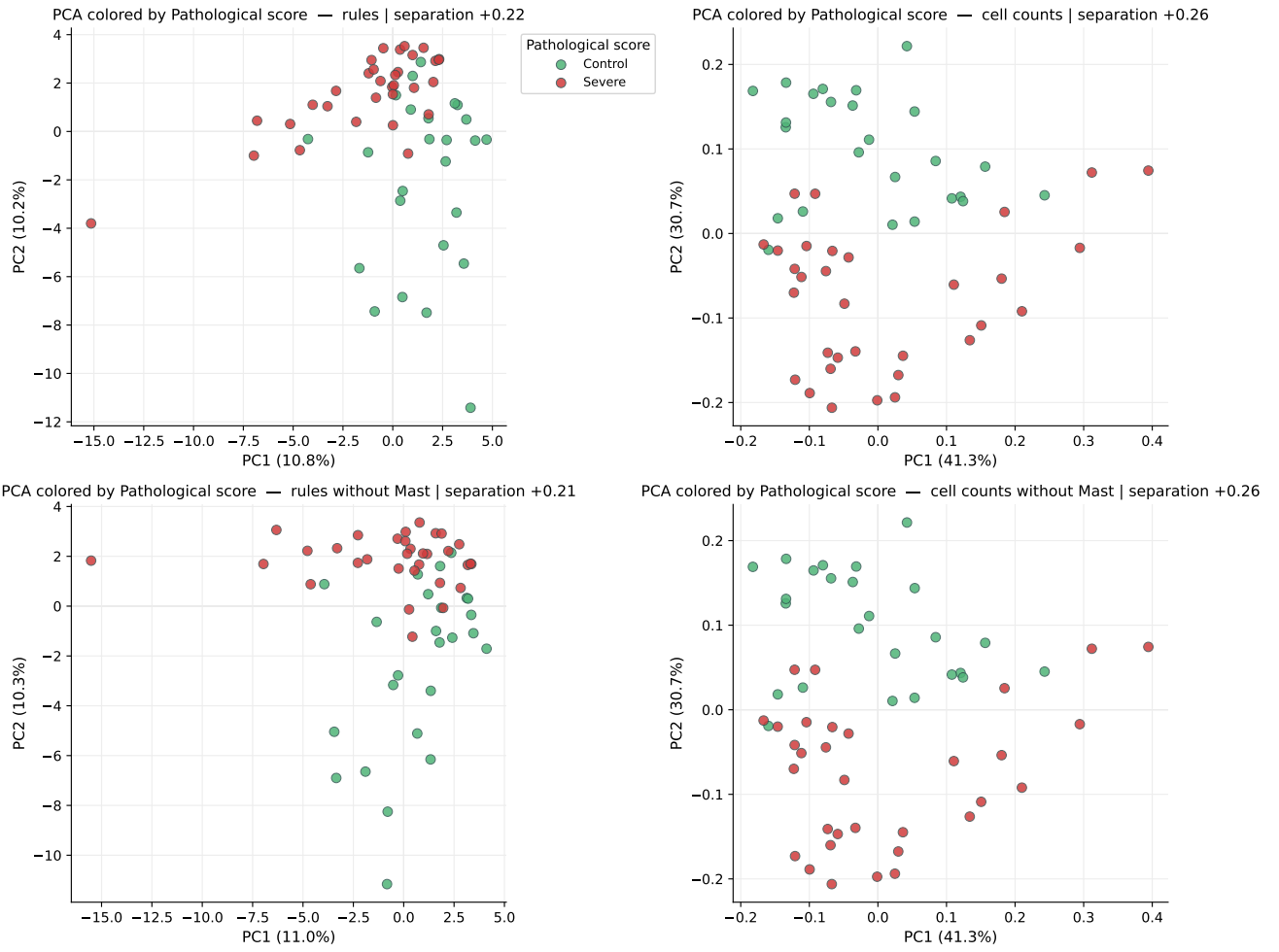
Figure 33: Values follow Figure 1.7; colon, Control against Severe, coloured by pathological score.
