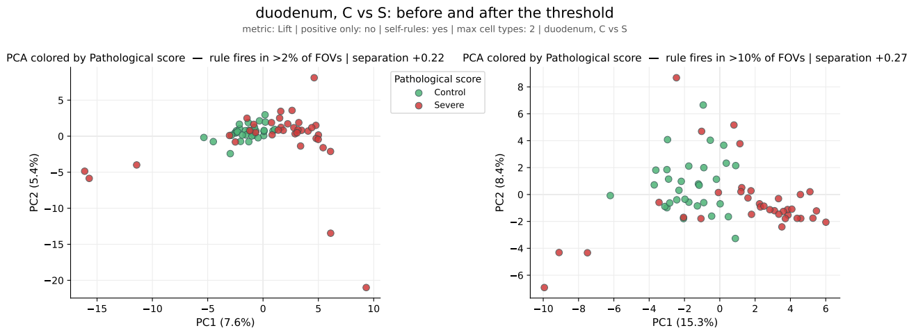
Figure 75: Duodenum, Control against Severe, at the old 2% threshold and at the 10% used here. Same FOVs and same colours; only the rule set differs, so each panel's axes are its own and only the grouping compares. On the left the FOVs are crushed into one clump because five far-out FOVs are stretching the axes; on the right they use the whole plot, and Control sits upper-left against Severe lower-right. Part of the gain is the outliers losing their grip on the scale, and part is a real separation — +0.22 to +0.27.
