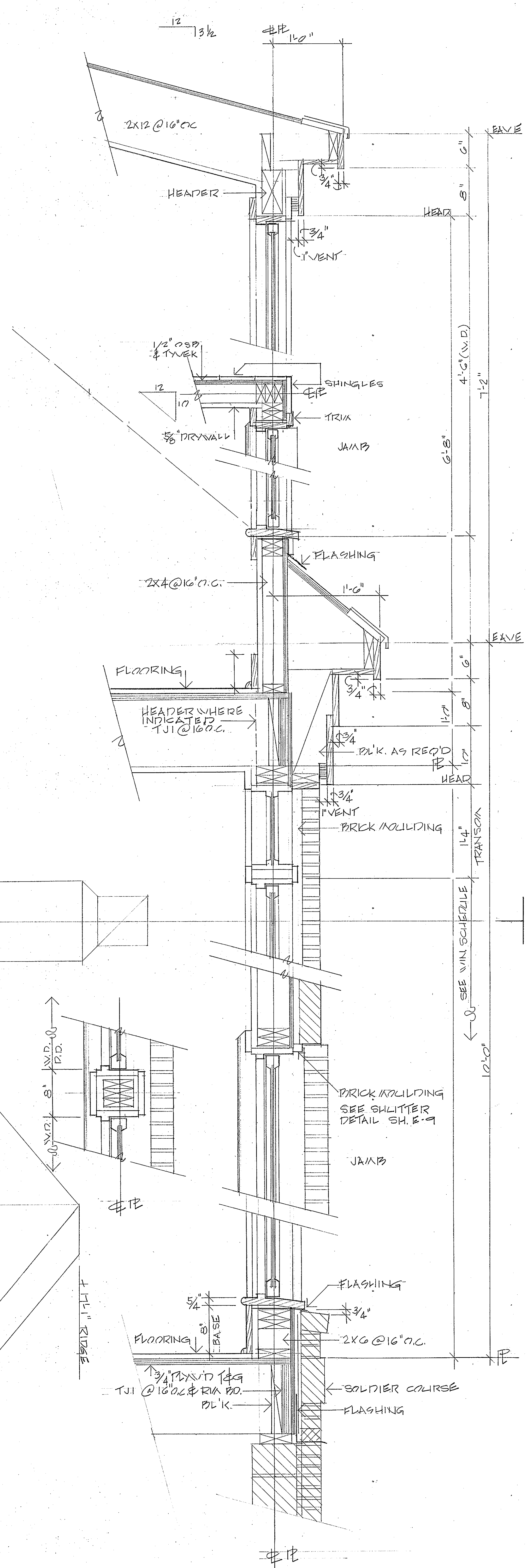
DETAIL SECTION 11/2"=1'-0"
