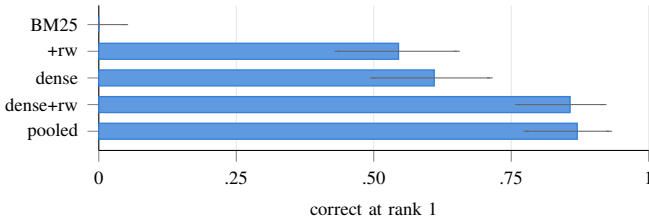
Fig. 2. The five retrieval configurations over 77 queries, with 95% Wilson score intervals [17]: BM25 0/77, with rewriting 42/77, dense 47/77, dense with rewriting 66/77, and the deployed pooling of both 67/77. Wilson intervals are asymmetric near the ends of the range, and are drawn as measured rather than symmetrised. The lexical baseline’s interval reaches only 0.048 and excludes every other configuration; the gap between rewriting and pooling is one query and their intervals almost coincide.
