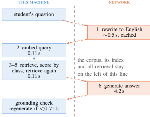
Fig. 1. The mandatory request path. Every figure is a median over 15 warm requests, five questions run three times, measured on the machine this work was developed on, an Apple M1 with 8 GB of memory. That is where the numbers were taken, not a requirement: the memory the platform needs is the 2,094 MB of Section VI, which is what puts it inside 4 GB. The dashed line is the machine boundary. Everything on its left, including the corpus and the whole of retrieval, stays on the machine; the two hosted calls are the only points at which a question leaves it, and the answer crosses back for grounding. Stages 3–5 are drawn as one box because they are three vector operations totalling \sim 0.05 s. Stage 6 produces a complete answer and is therefore slower than the fixed short completion used for model selection (Table III). Generation dominates and is the least predictable stage, at 4.2 s median against a 95th percentile of 13.2 s, because it is a call to a hosted endpoint. The rewrite is cached, so a repeated question pays nothing for it and a new one pays about half a second. Retrieval is 0.11 s for all three of its stages together. The grounding check carries no latency because we did not measure it separately. The two optional stages, reading support and illustration, are omitted here. Without them a warm request completes in 4.4 s at the median.
