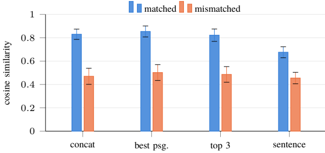
Fig. 5. Four grounding estimators over 16 matched and 240 mismatched pairs, with one standard deviation. What separates the populations is the distance between the two bars, not the height of either. Scoring against the single best passage raises both means without widening that distance, and scoring sentence by sentence narrows it.
