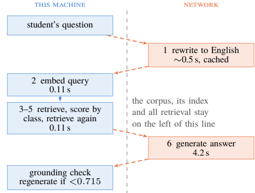
Fig. 1. The mandatory request path. Medians over 15 warm requests, five questions run three times on an 8 GB Apple M1. The dashed line is the machine boundary: the corpus and all retrieval stay left of it. Generation dominates and is least predictable, 4.2 s median against a 95th percentile of 13.2 s, because it is hosted. All of retrieval is 0.11 s. The grounding check carries no latency because it was not measured separately.
