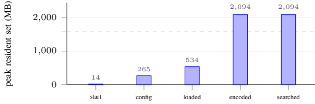
Fig. 4. Peak resident set through the serving pipeline, from interpreter start through configuration import, model load, the first query encoding, and a completed vector search. The dashed line is the 1,600 MB an earlier analysis predicted by summing component sizes. Loading the weights accounts for 534 MB because safetensors memory-maps them; the 1,560 MB that follows arrives on the first forward pass, when those pages become resident and the attention workspaces are allocated.
