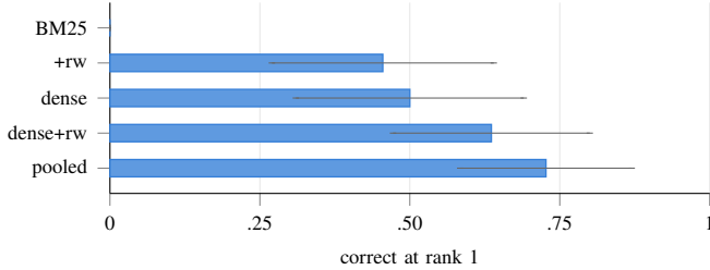
Fig. 2. The five retrieval configurations over 22 queries, with 95% Wilson score intervals [17]: BM25 0/22, with rewriting 10/22, dense 11/22, dense with rewriting 14/22, and the deployed pooling of both 16/22. The intervals overlap across the three dense configurations, which is why this paper claims an ordering and not a margin. The lexical baseline’s interval excludes all three, and no sample-size argument softens that.
