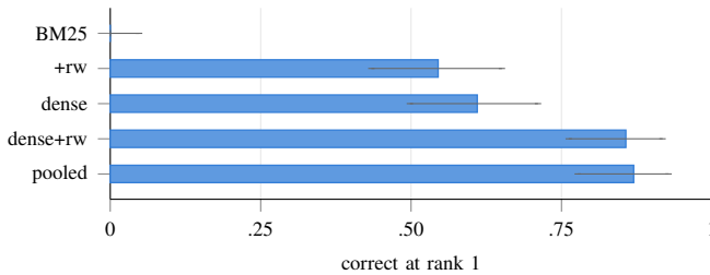
Fig. 2. The five retrieval configurations over 77 queries, with 95% Wilson score intervals [18]: BM25 0/77, with rewriting 42/77, dense 47/77, dense with rewriting 66/77, and the deployed pooling of both 67/77. Wilson intervals are asymmetric near the ends of the range, and are drawn as measured rather than symmetrised. The lexical baseline’s interval reaches only 0.048 and excludes every other configuration; the gap between rewriting and pooling is one query and their intervals almost coincide.
