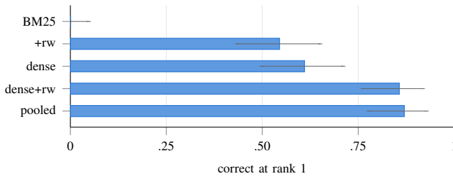
Fig. 2. The five retrieval configurations over 77 queries, with 95% Wilson score intervals [17]: BM25 0/77, with rewriting 42/77, dense 47/77, dense with rewriting 66/77, and the deployed pooling of both 67/77. Wilson intervals are asymmetric near the ends of the range, and are drawn as measured rather than symmetrised. The lexical baseline’s interval reaches only 0.048 and excludes every other configuration; the gap between rewriting and pooling is one query and their intervals almost coincide.
