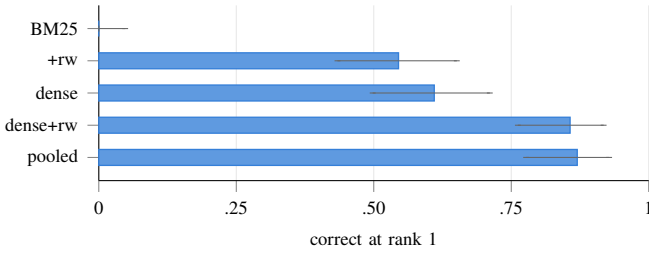
Fig. 2. The five retrieval configurations over 77 queries, with 95% Wilson score intervals [25]: BM25 0/77, with rewriting 42/77, dense 47/77, dense with rewriting 66/77, and the deployed pooling of both 67/77. Wilson intervals are asymmetric near the ends of the range, and are drawn as measured rather than symmetrised. The lexical baseline’s interval reaches only 0.048 and excludes every other configuration; the gap between rewriting and pooling is one query and their intervals almost coincide.
