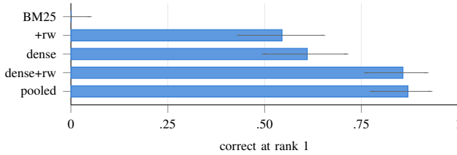
Fig. 2. The five retrieval configurations over 77 queries, with 95% Wilson score intervals [18]: BM25 0/77, with rewriting 42/77, dense 47/77, dense with rewriting 66/77, and the deployed pooling of both 67/77. Wilson intervals are asymmetric near the ends of the range, and are drawn as measured rather than symmetrised. The lexical baseline’s interval reaches only 0.048 and excludes every other configuration; the gap between rewriting and pooling is one query and their intervals almost coincide.
