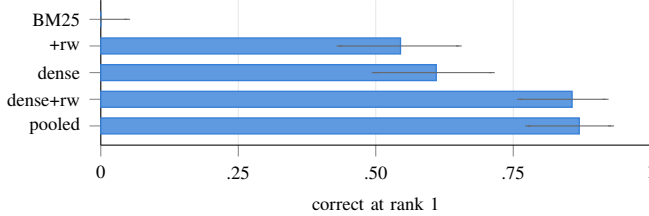
Fig. 2. The five retrieval configurations over 77 queries, with 95% Wilson score intervals [17]: BM25 0/77, with rewriting 42/77, dense 47/77, dense with rewriting 66/77, and the deployed pooling of both 67/77. Wilson intervals are asymmetric near the ends of the range, and are drawn as measured rather than symmetrised. The lexical baseline’s interval reaches only 0.048 and excludes every other configuration; the gap between rewriting and pooling is one query and their intervals almost coincide.
