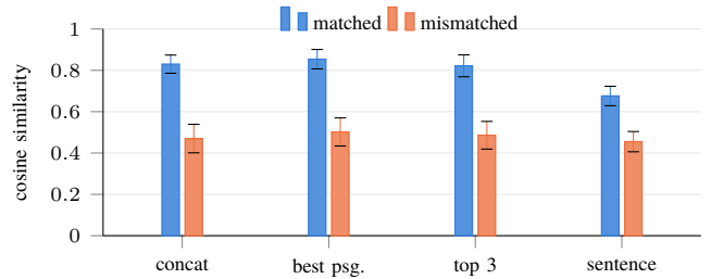
Fig. 4. Four grounding estimators over 16 matched and 240 mismatched pairs, with one standard deviation. What separates the populations is the distance between the two bars. Their heights do not matter.
