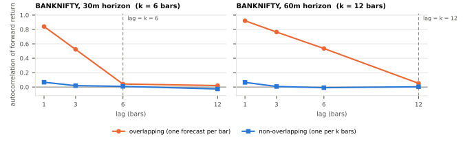
Fig. 1. Forward-return autocorrelation, overlapping versus non-overlapping, at two horizons. The overlapping series dies at exactly lag k in both panels.
