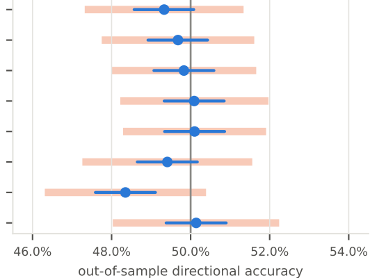
NIFTY50 (24,075 bars, 5 purged folds)
