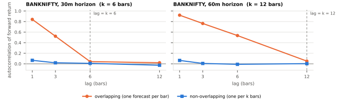
Fig. 1. Forward-return autocorrelation, overlapping versus non-overlapping, at two horizons. The overlapping series dies at exactly lag k in both panels.
