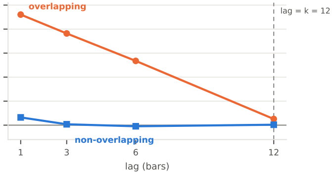
BANKNIFTY, 60m horizon (k = 12 bars)
