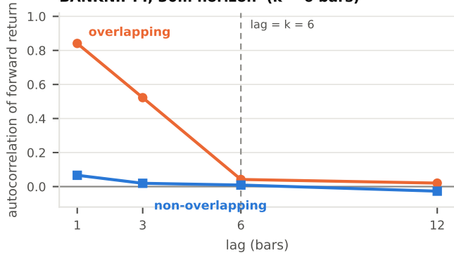
BANKNIFTY, 30m horizon (k = 6 bars)
