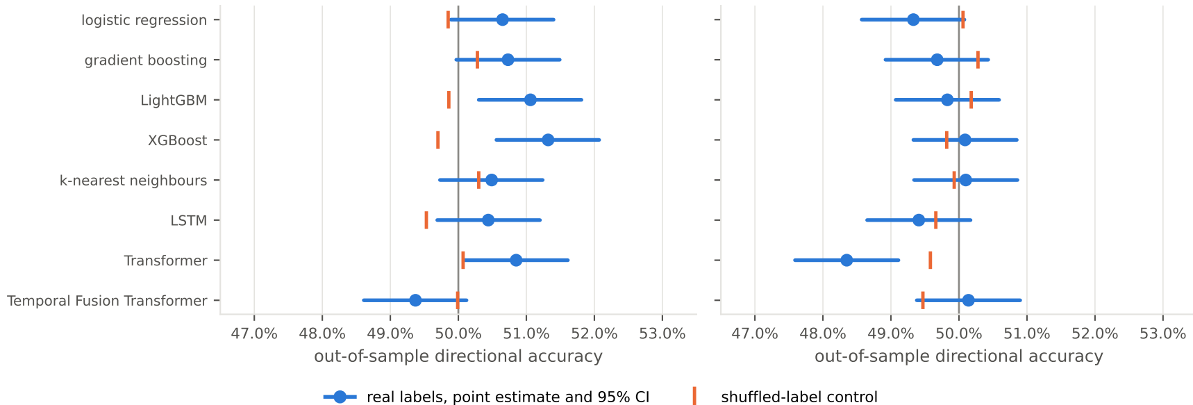
BANKNIFTY (24,080 bars, 5 purged folds)
