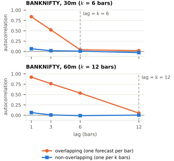
Fig. 1. Forward-return autocorrelation, overlapping versus non-overlapping, at two horizons. The overlapping series dies at exactly lag k in both panels.
