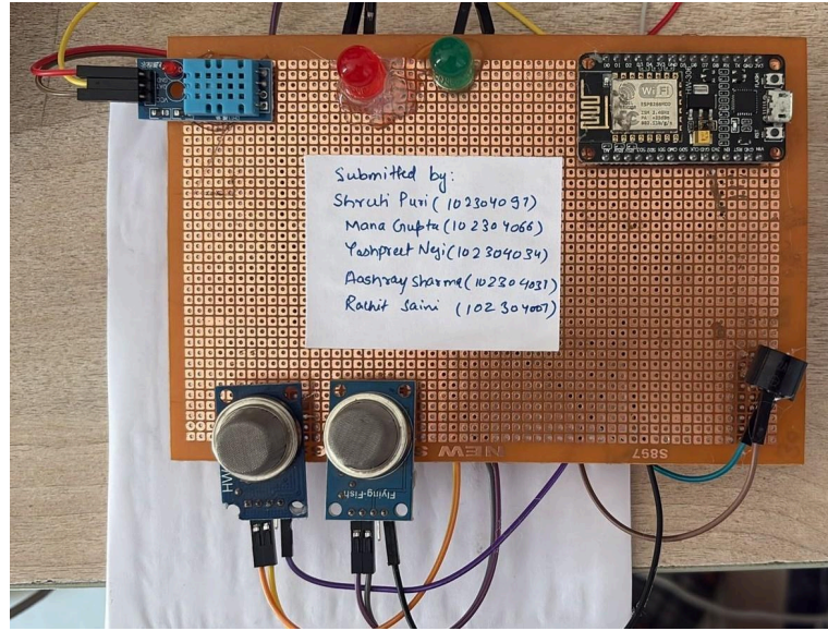
Figure 4: Assembled prototype of the AQI sensor module on the PCB.
