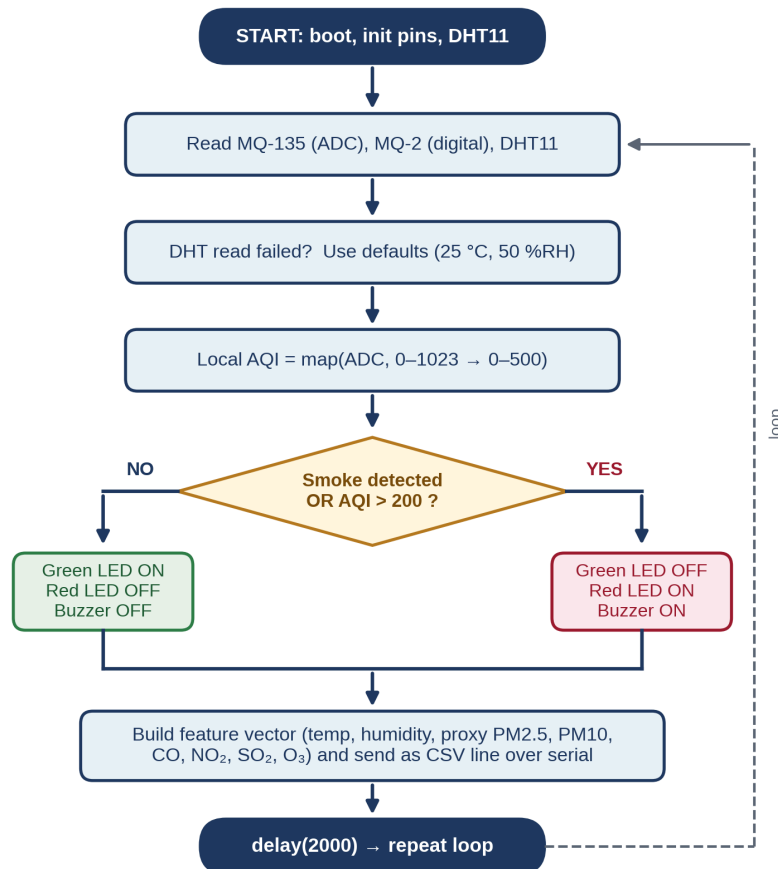
Figure 6: Flowchart of the ESP8266 firmware loop.
