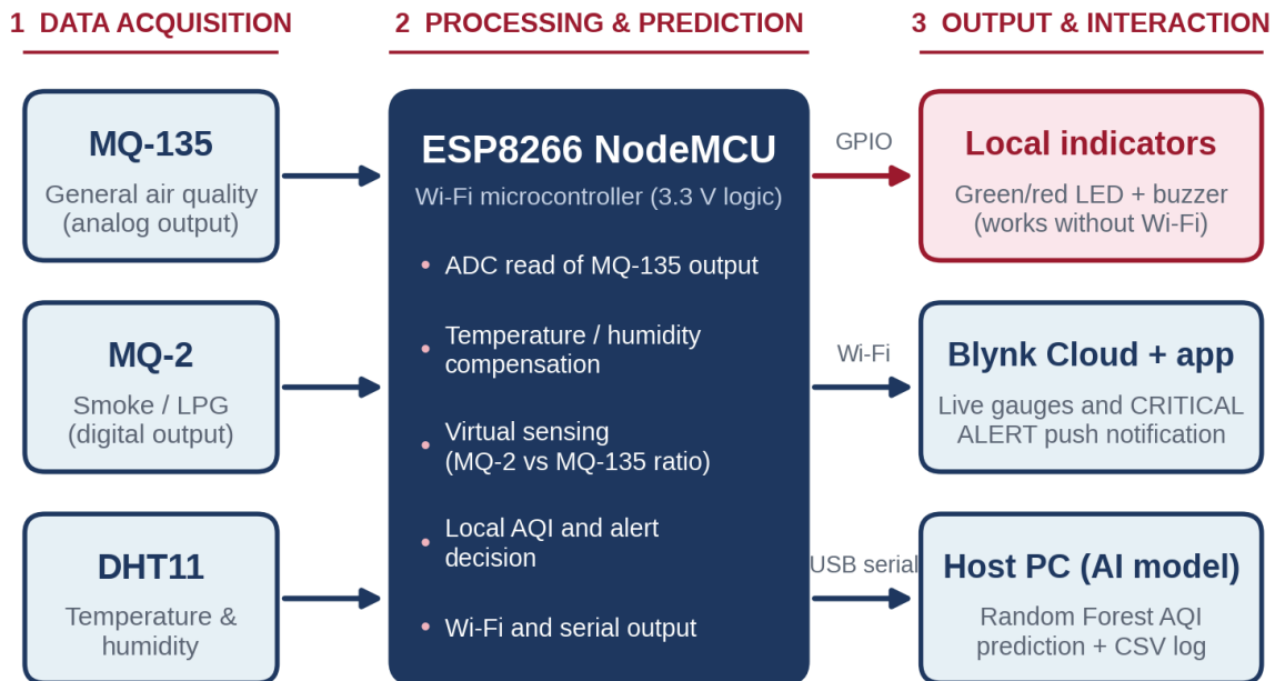
Figure 1: Overall system architecture of the AI-reinforced AQI sensor module.
