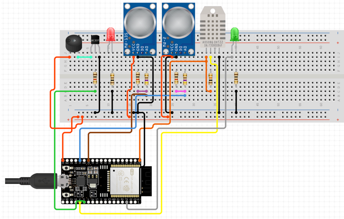
Figure 5: Breadboard wiring diagram of the sensor module (sensor interfacing, indicators and buzzer driver).
