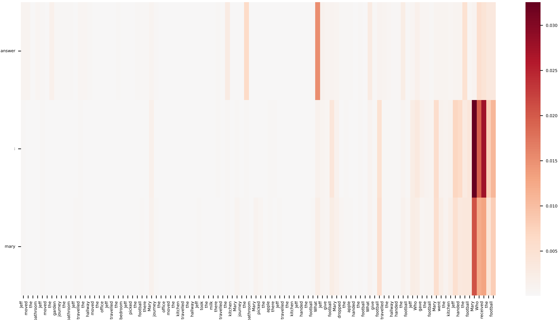
Task Tokens
