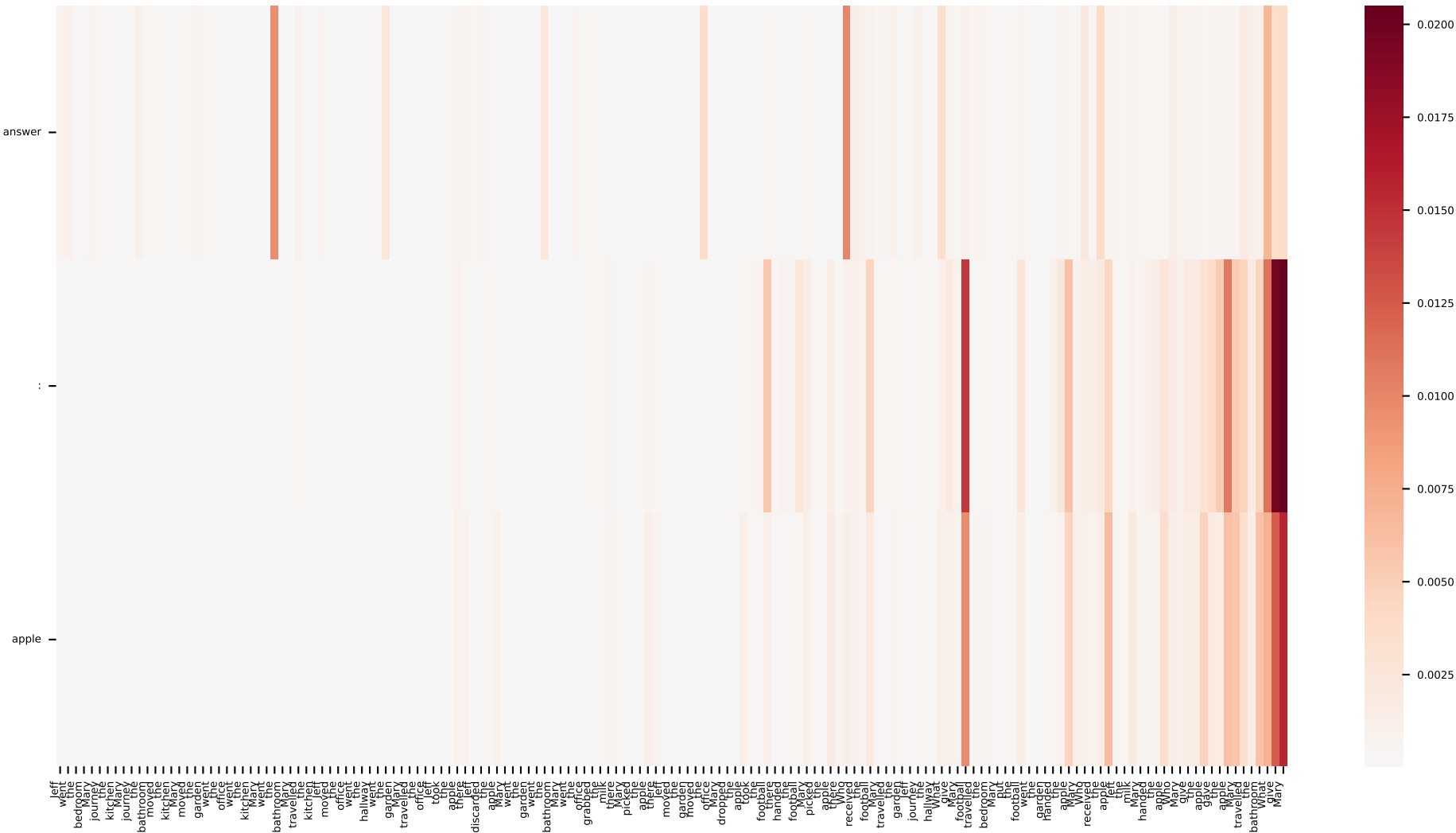
Task Tokens
