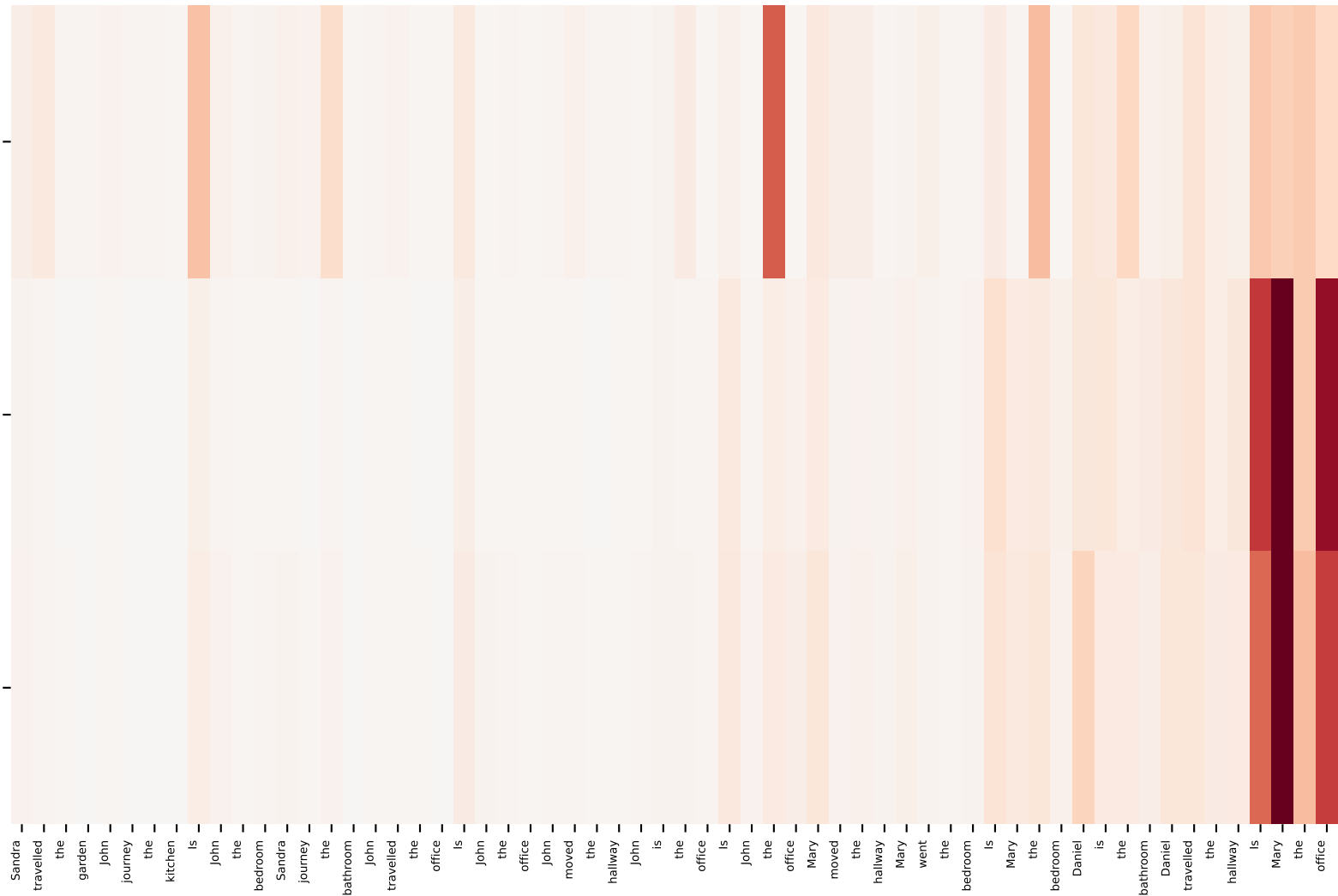
Task Tokens
