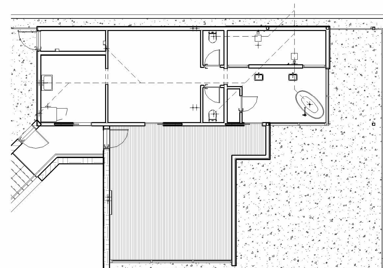
② 3-Upper Plumbing 1/8" = 1'-0"
