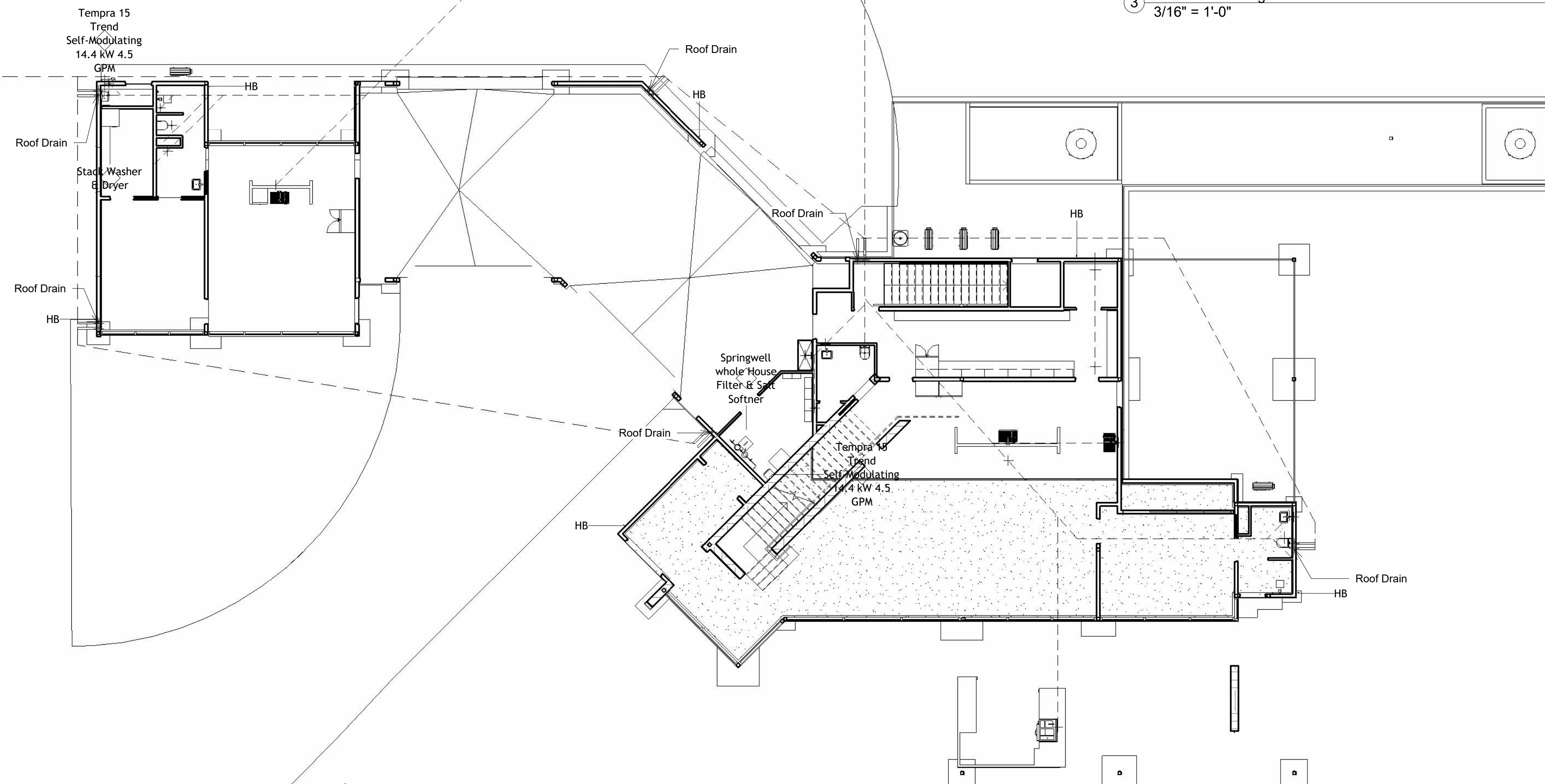
③ 4-Lower Plumbing 3/16" = 1'-0"
