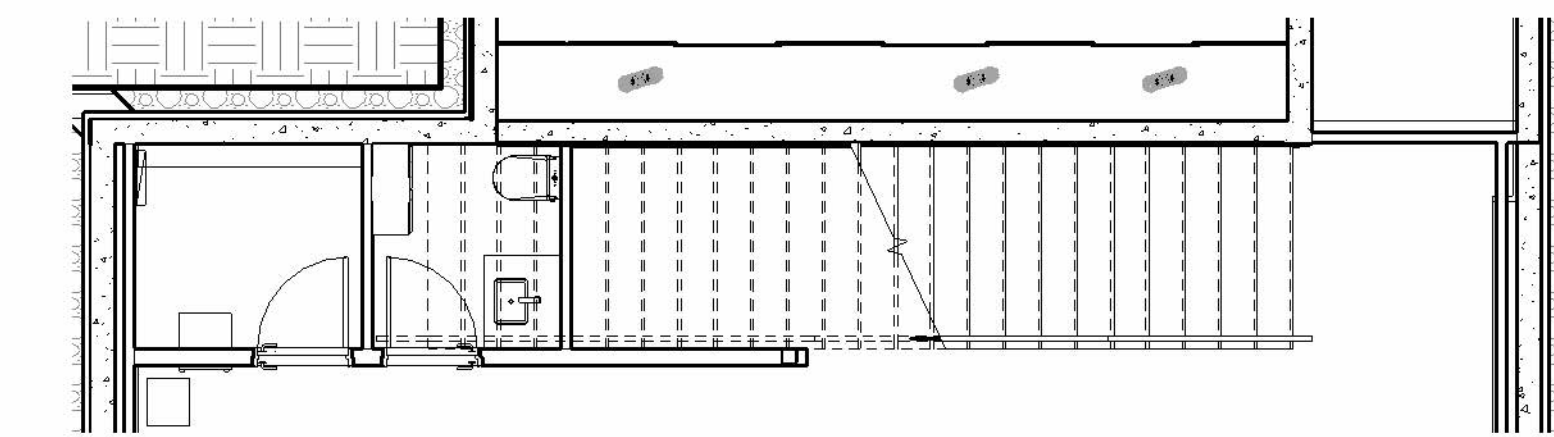
③ 4-Lower Plumbing 3/16" = 1'-0"
