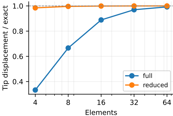
Slenderness L/h = 10
