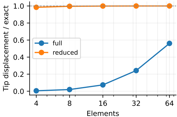
Slenderness L/h = 100
