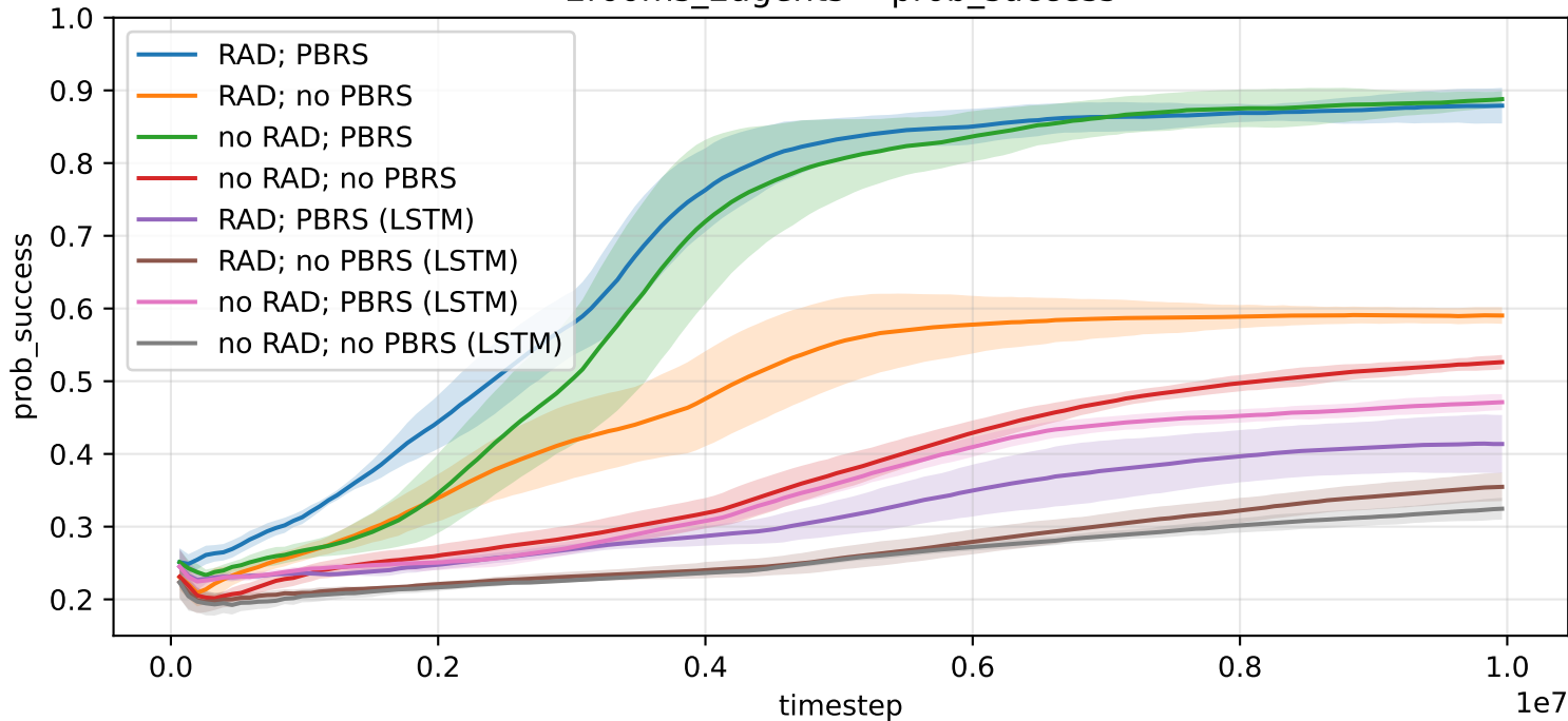
2rooms_2agents -- probab_success
