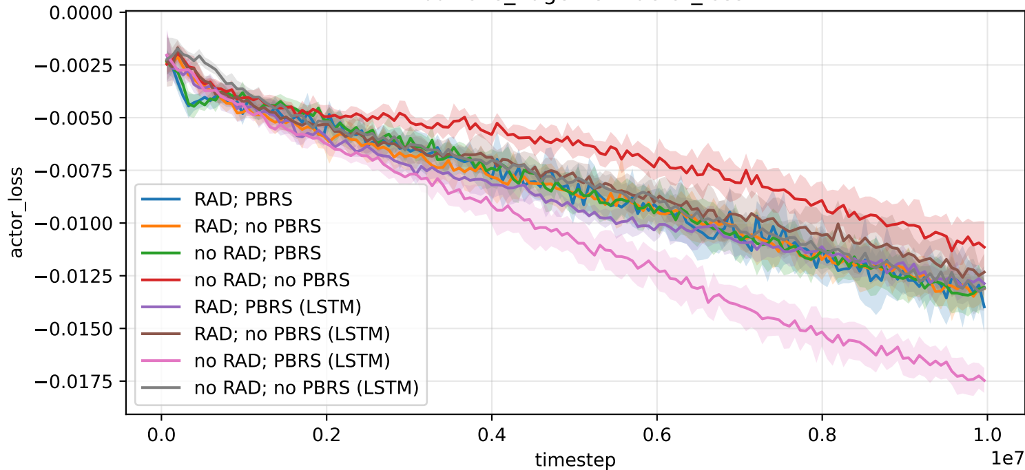
2buttons_2agents -- actor_loss
