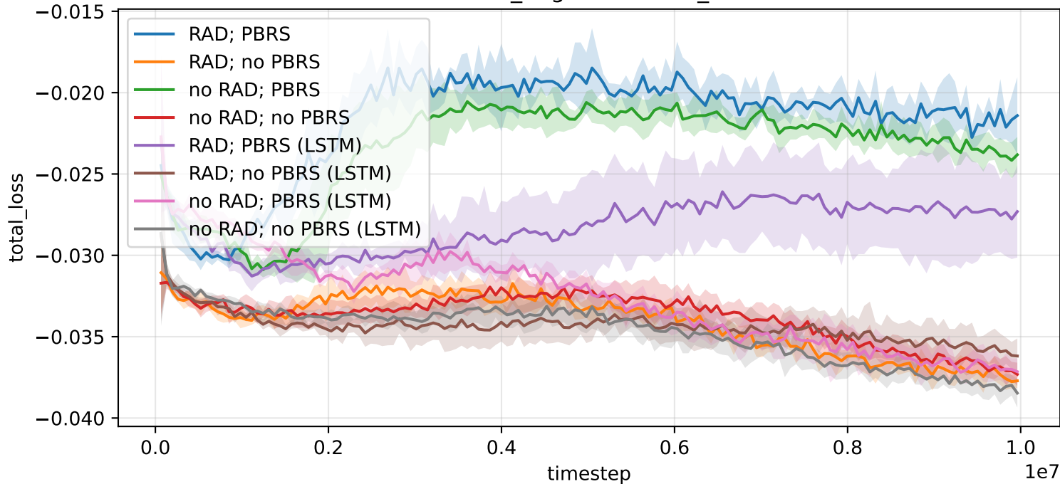
2rooms_2agents -- total_loss
