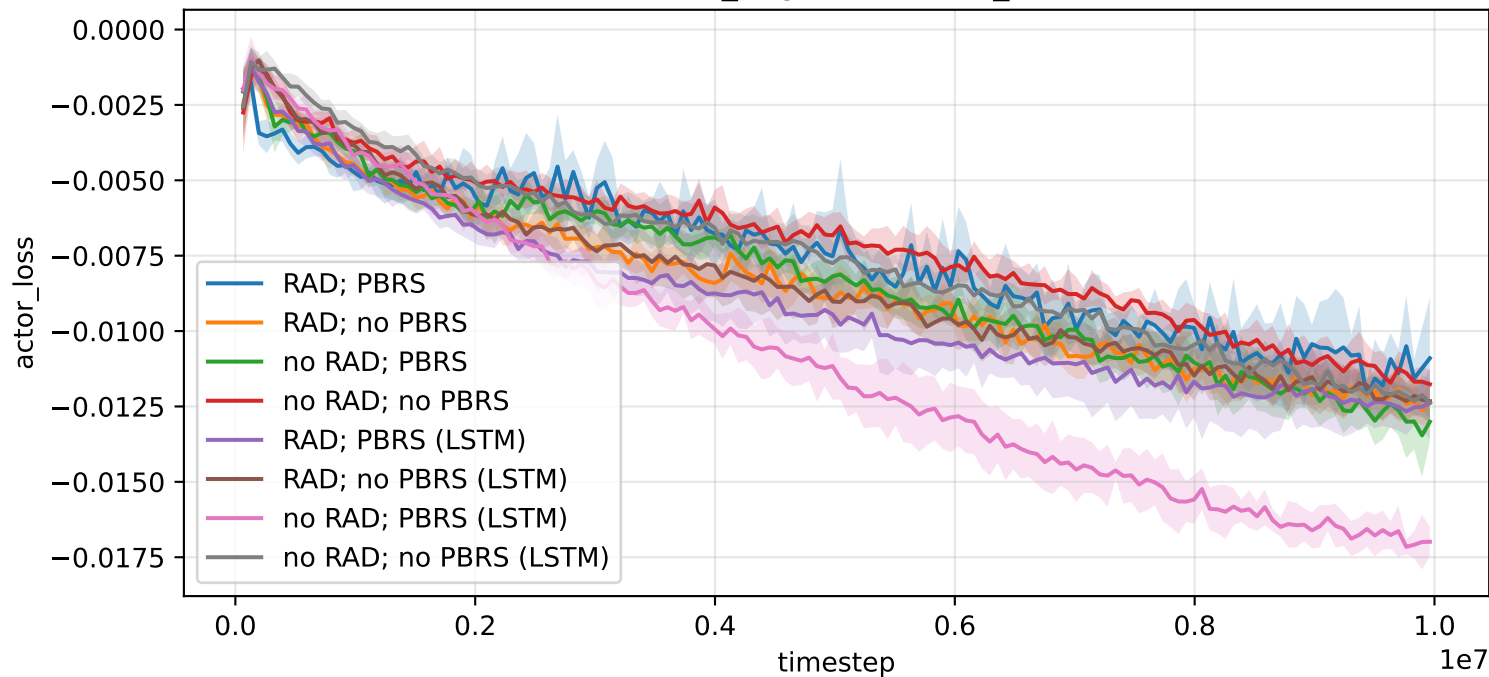
2rooms_2agents -- actor_loss
