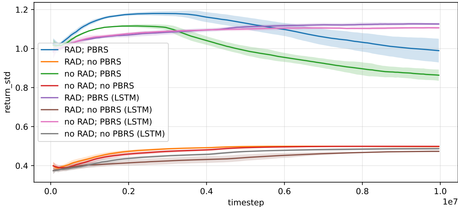
2buttons_2agents -- return_std
