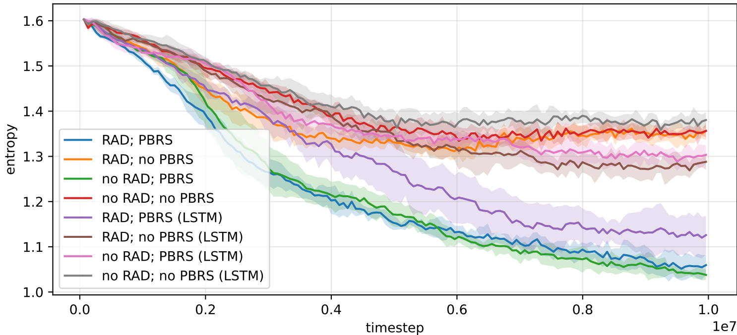
2rooms_2agents -- entropy
