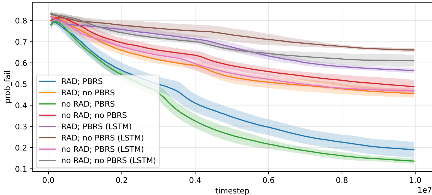
2buttons_2agents -- probab_fail
