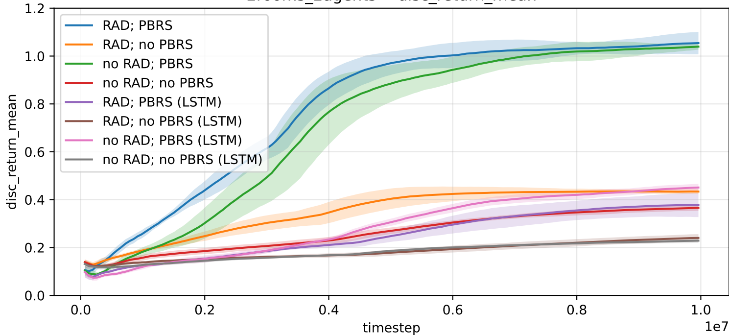
2rooms_2agents -- disc_return_mean
