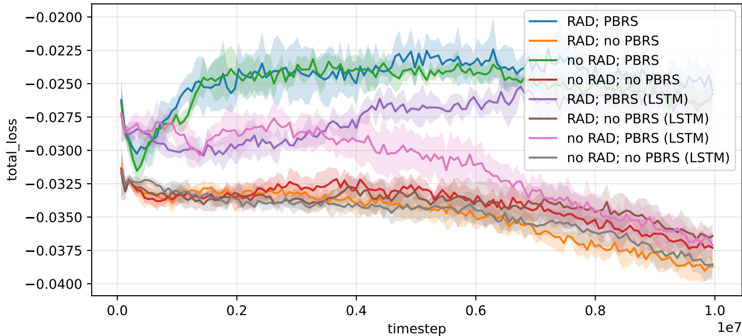
2buttons_2agents -- total_loss
