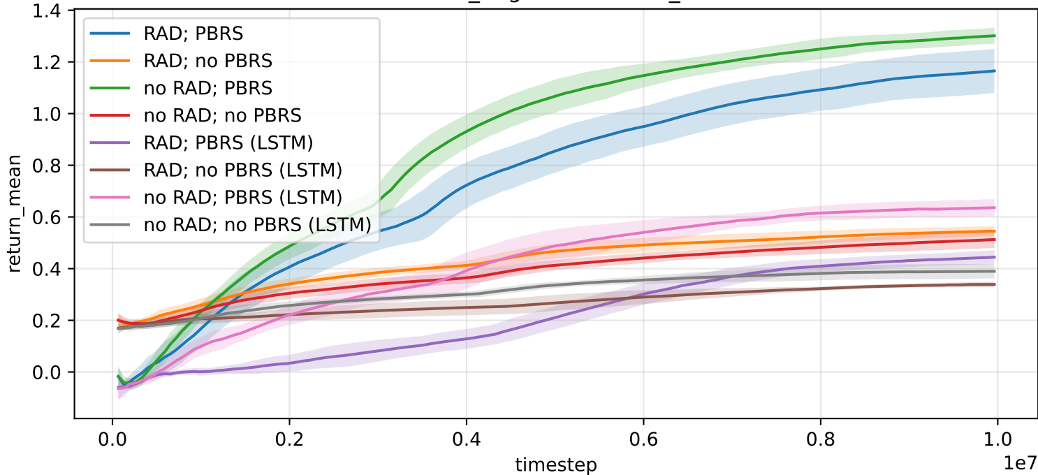
2buttons_2agents -- return_mean
