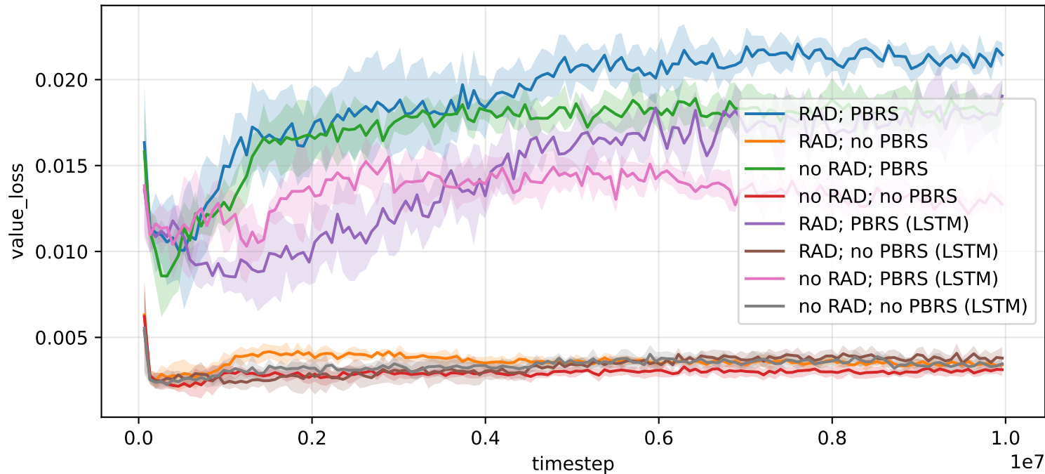
2buttons_2agents -- value_loss
