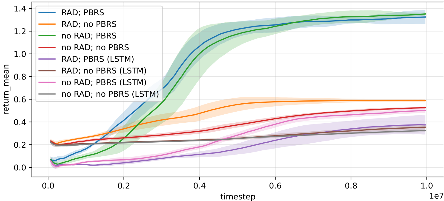
2rooms_2agents -- return_mean
