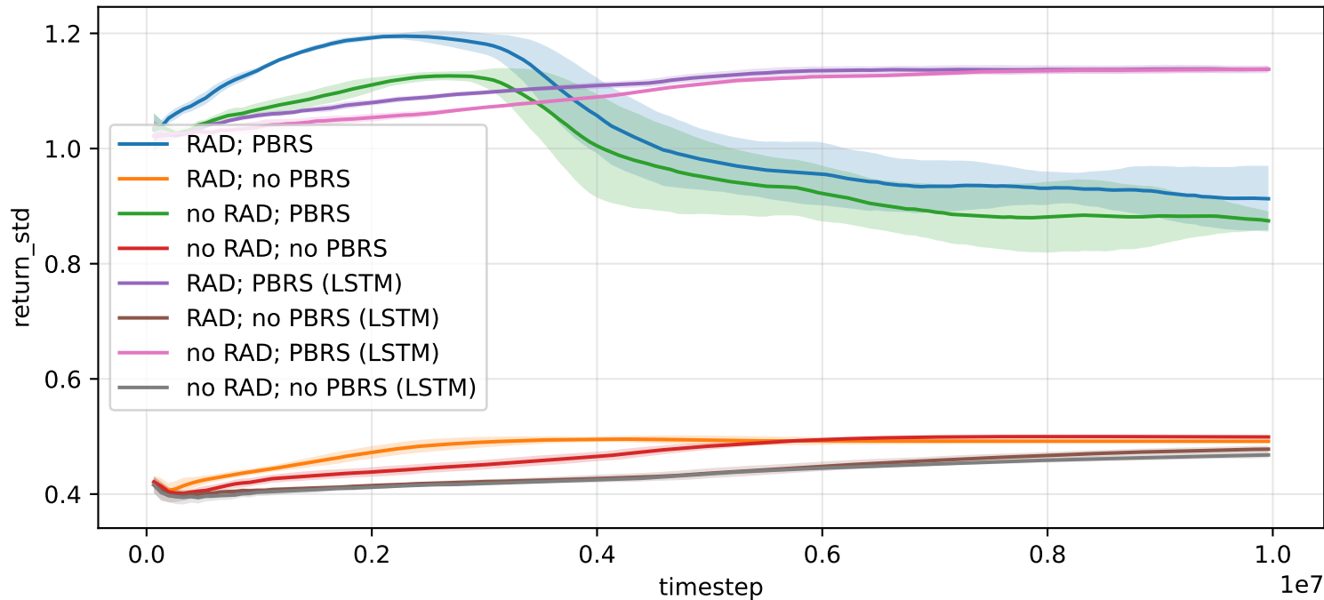
2rooms_2agents -- return_std
