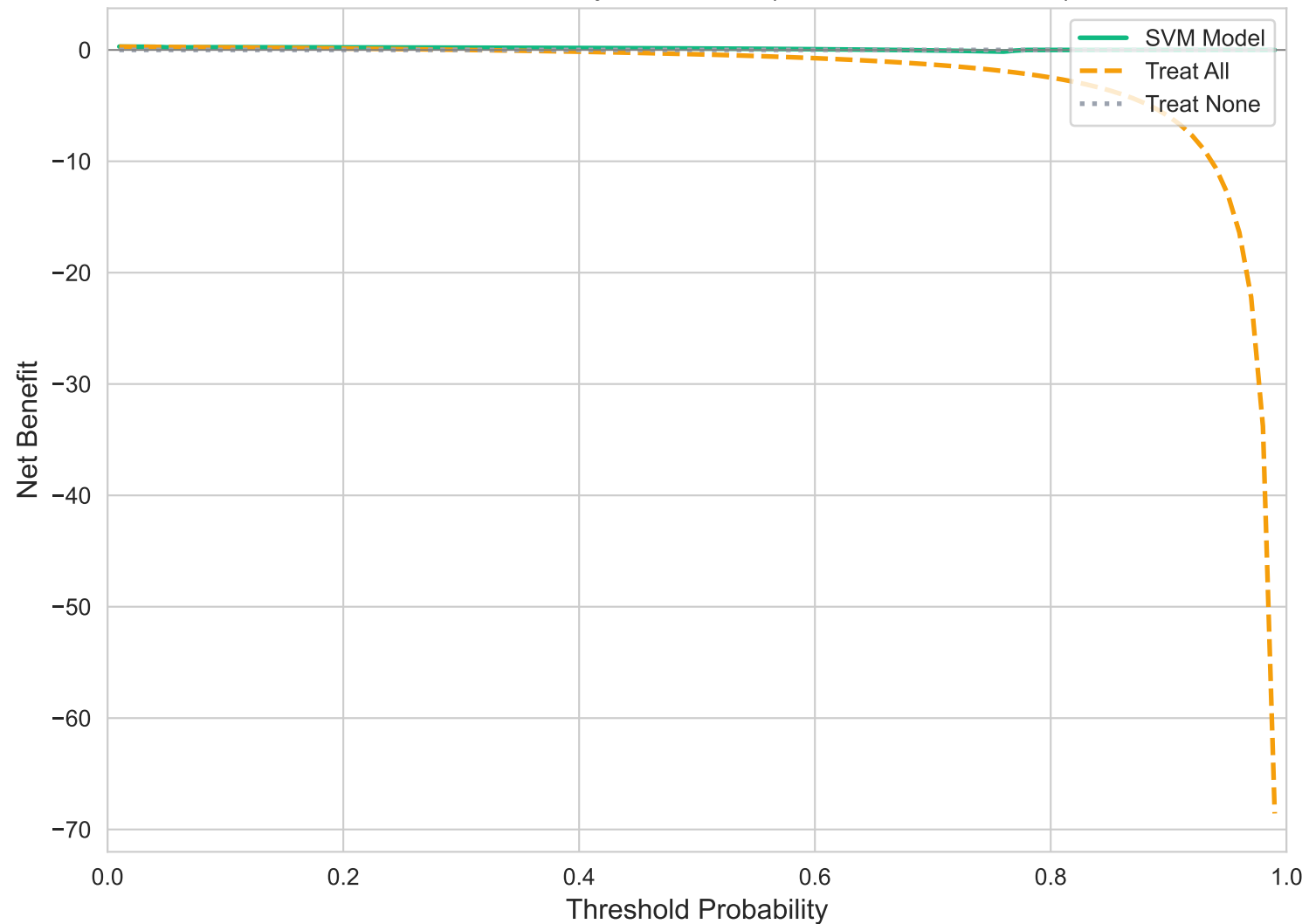
Decision Curve Analysis — SVM (Vickers & Elkin, 2006)
