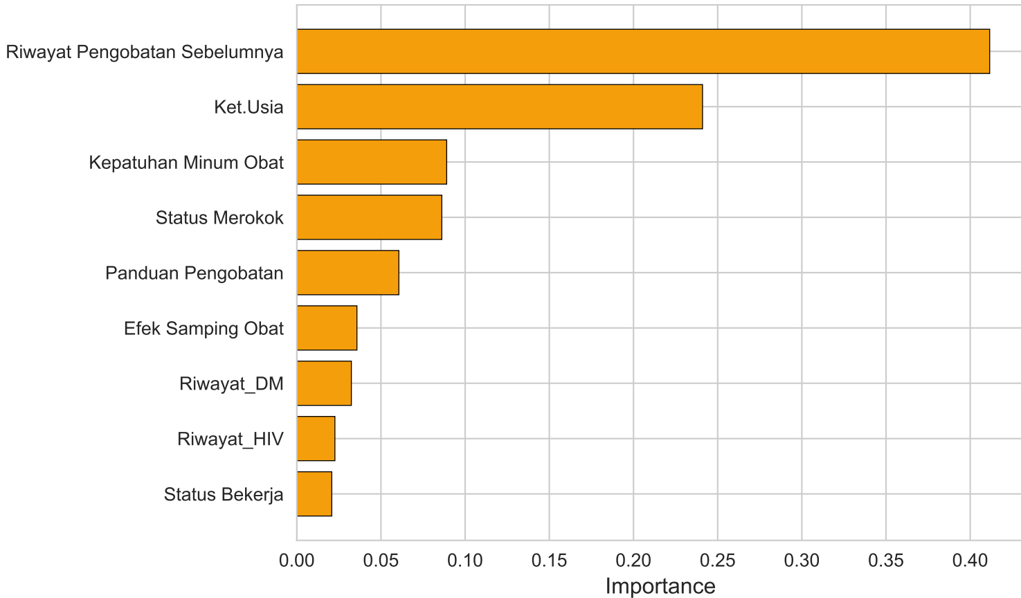
Feature Importance — Decision Tree
