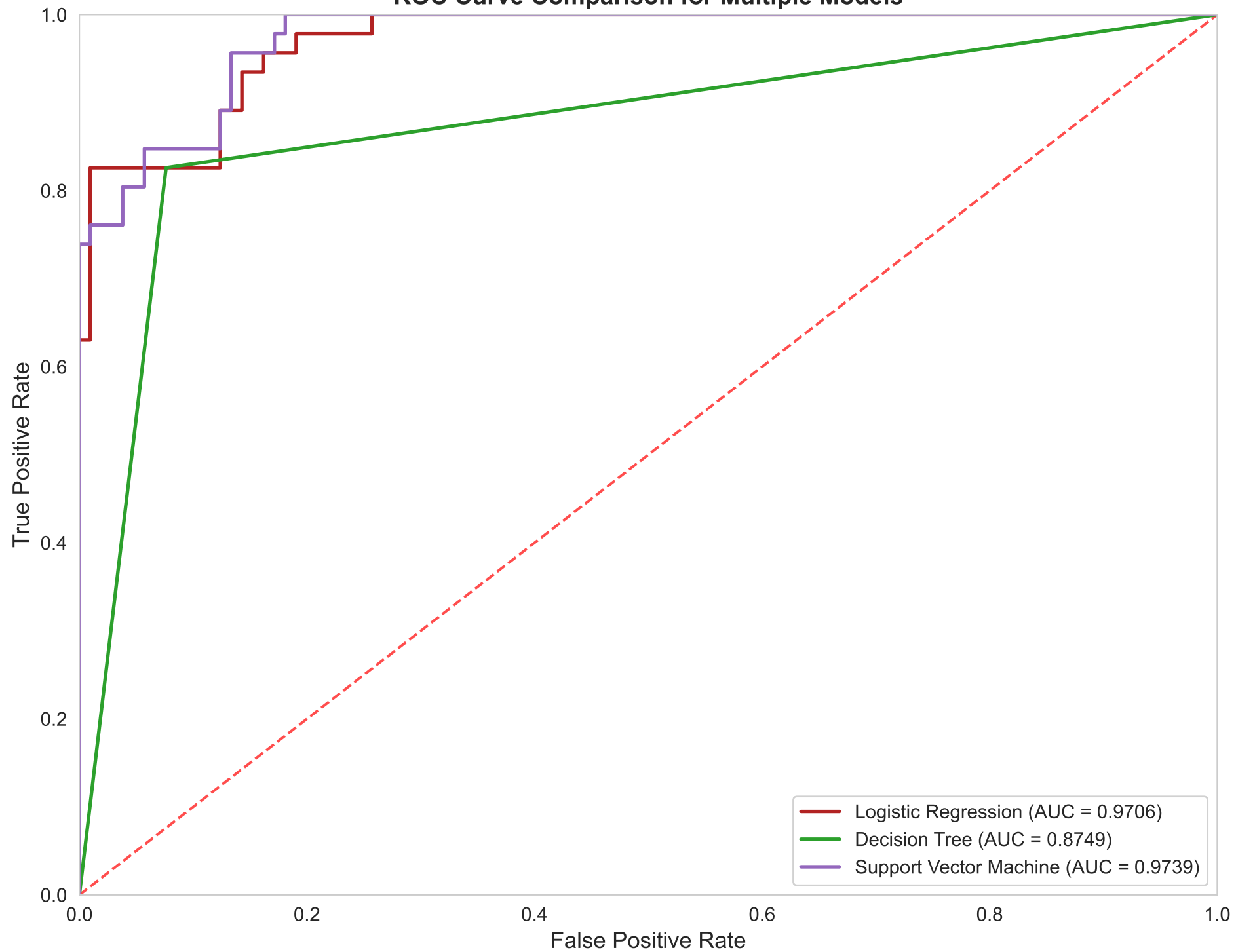
ROC Curve Comparison for Multiple Models
