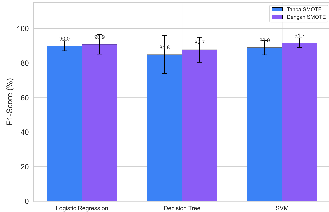
F1-Score
