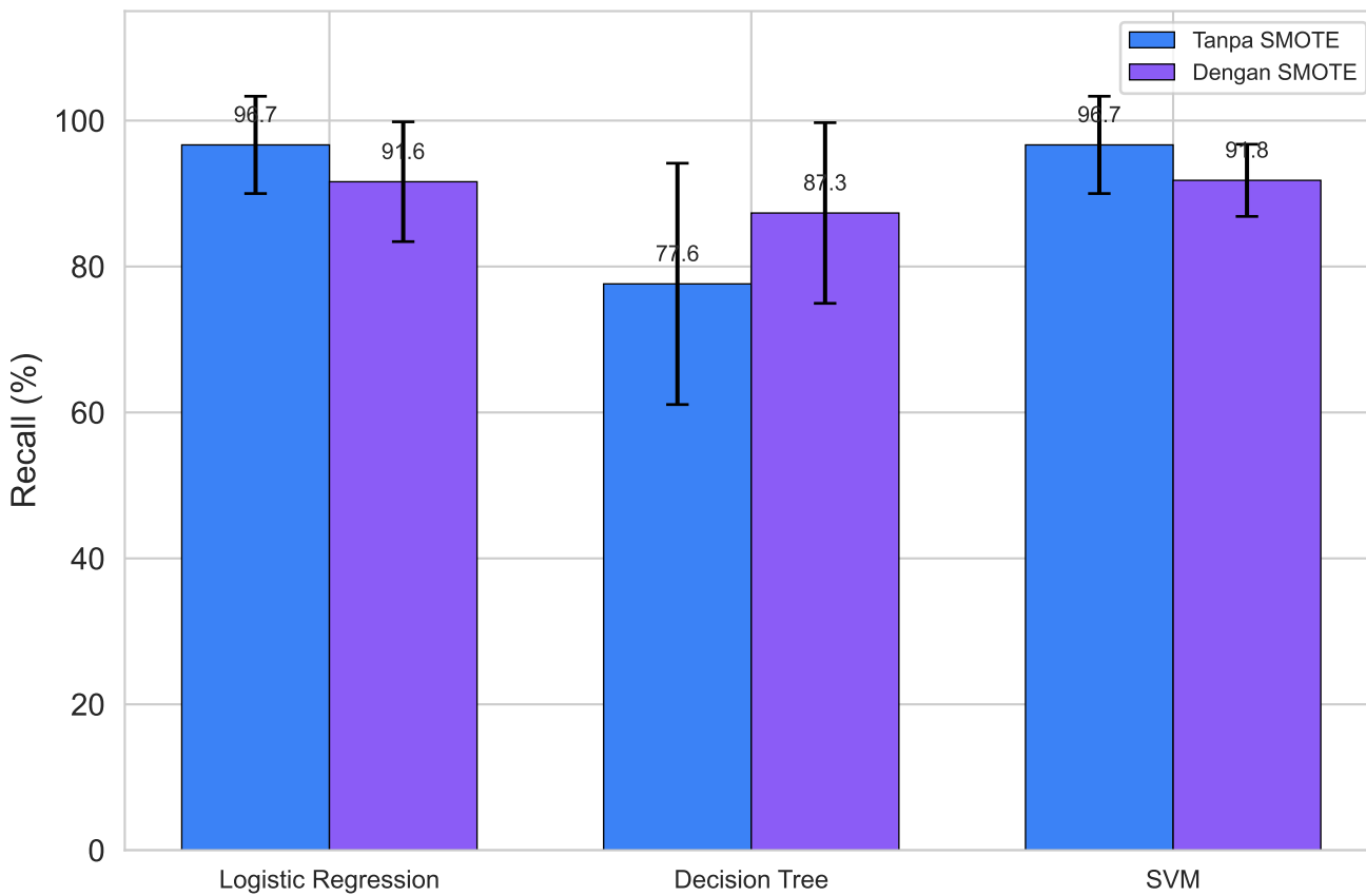
Recall
